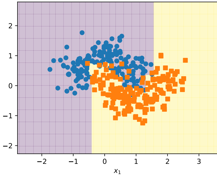
Decision Tree
