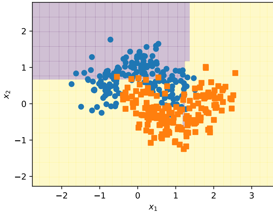
Extra Tree
