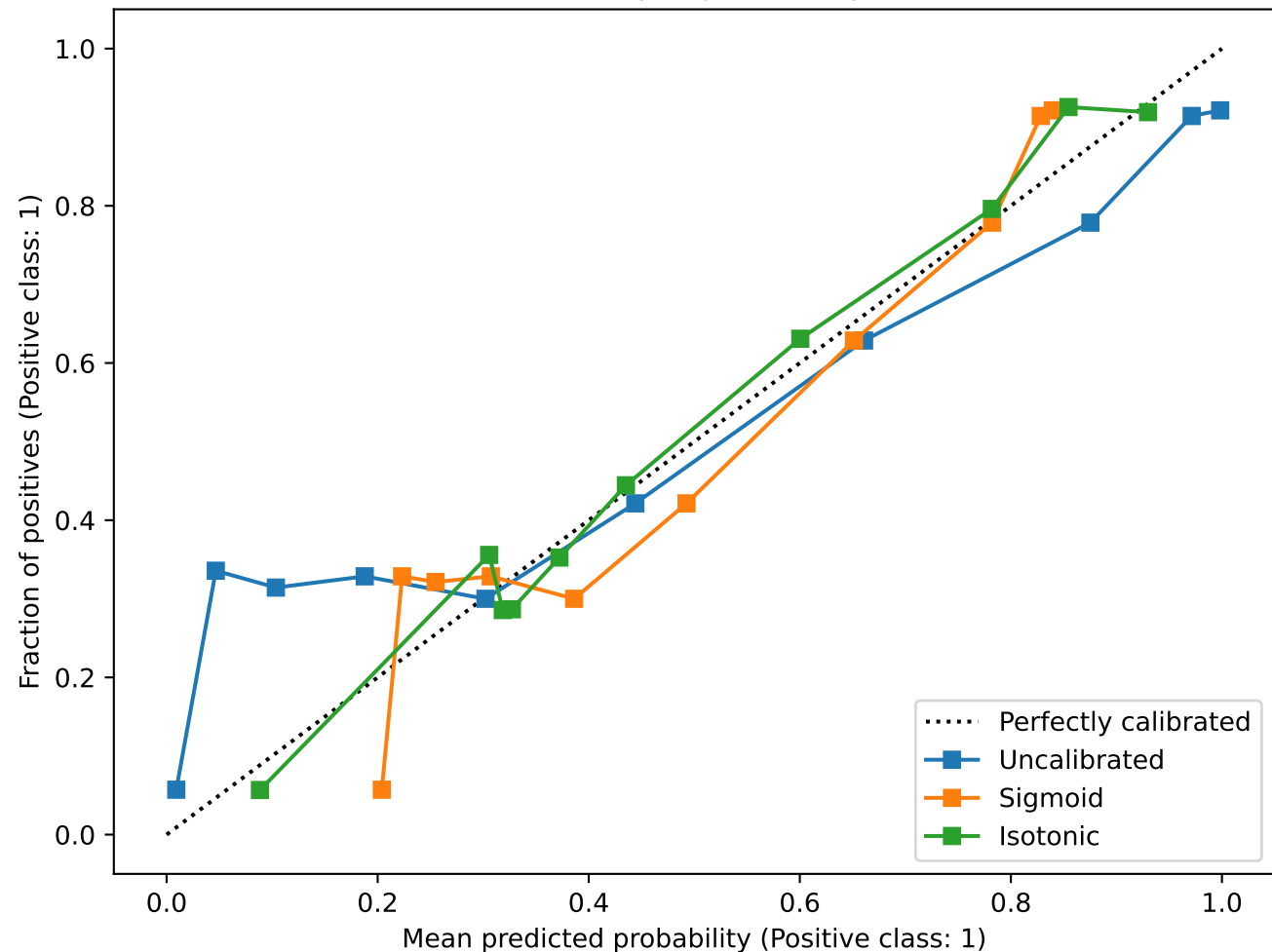
Gaussian Naive Bayes probability calibration
