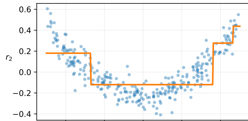
Stage 3 negative gradient and h_3(x)
