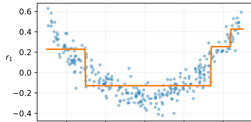
Stage 2 negative gradient and h_2(x)
