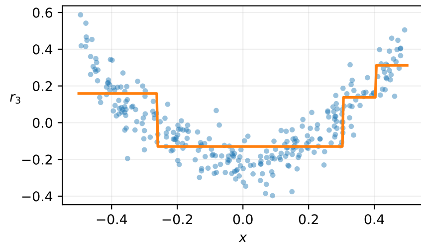
Stage 3 negative gradient and h_3(x)
