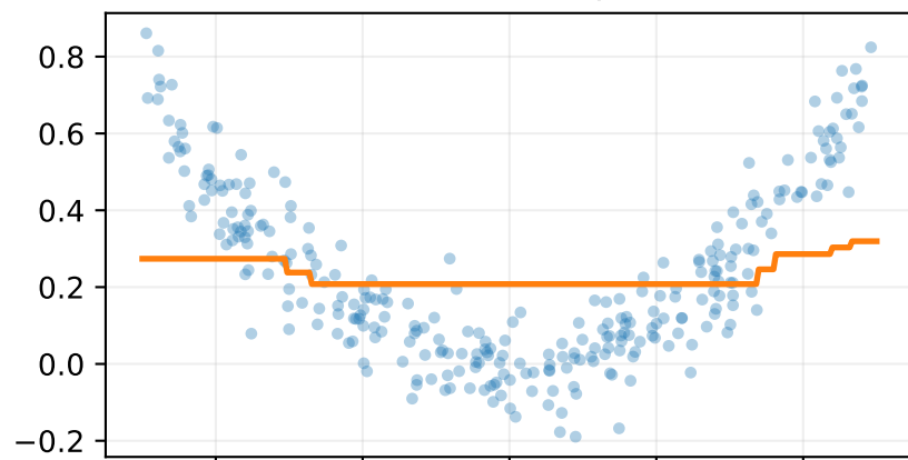
F_3(x) = F_2(x) + \eta h_3(x)
