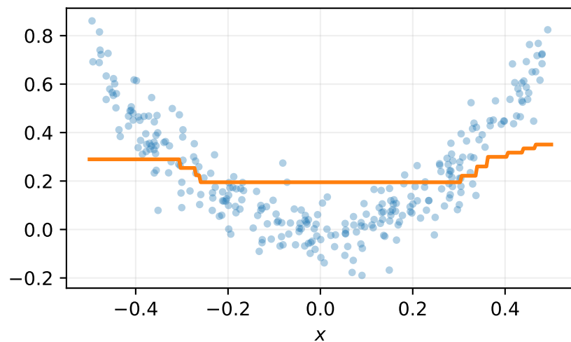
F_3(x) = F_2(x) + \eta h_3(x)
