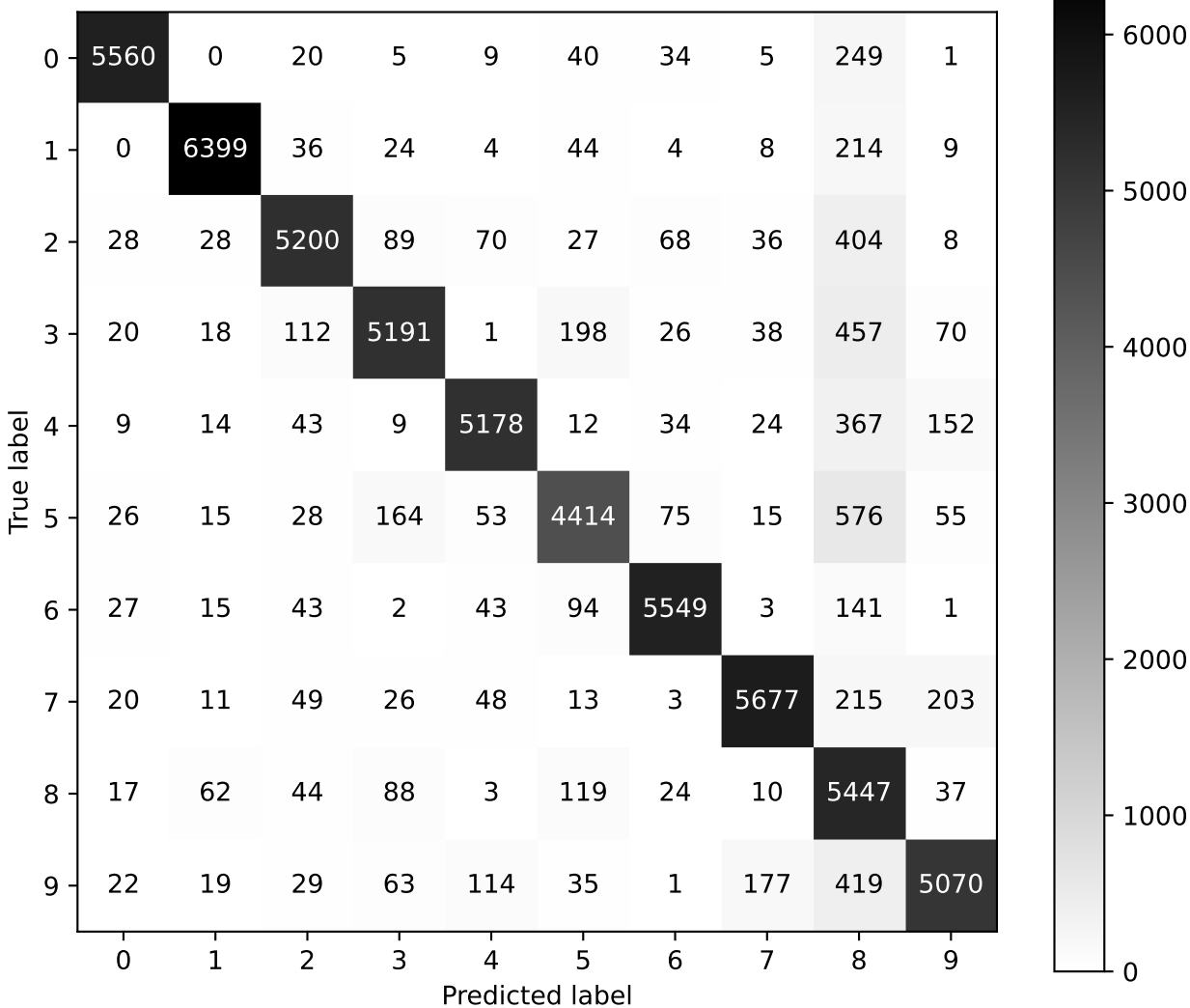
Confusion Matrix: SGD Classifier
