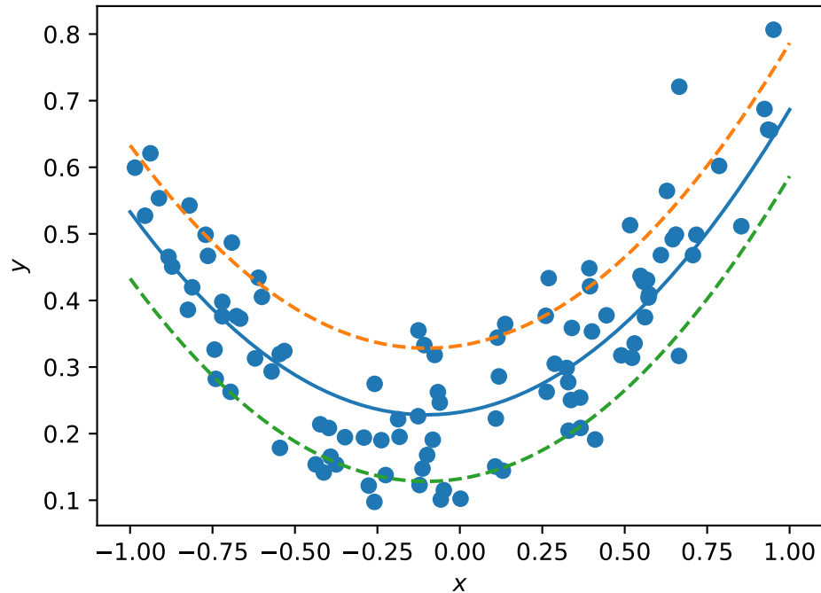
Polynomial SVR, C = 0.01
