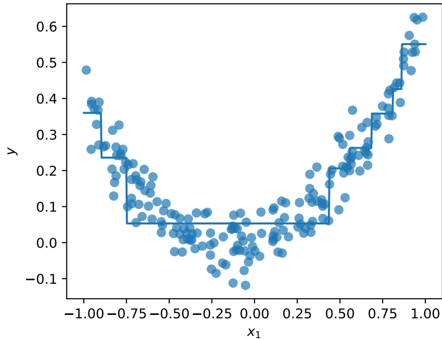
max_depth = 3
