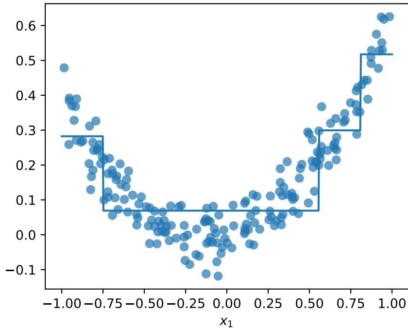
max_depth = 2
