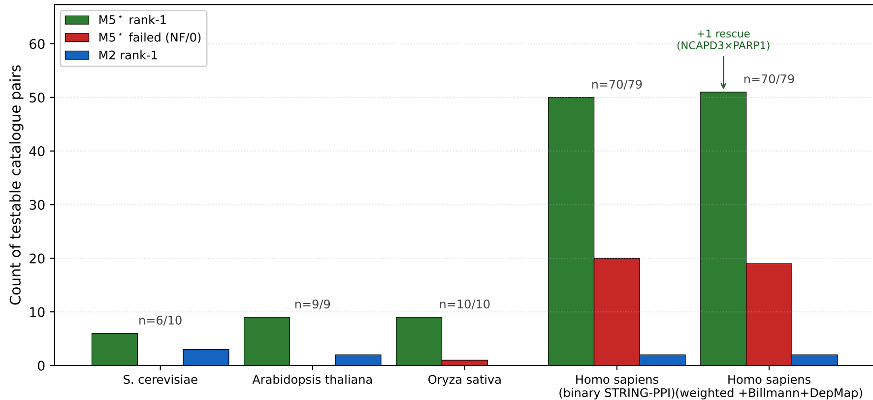
§Y.8 catalogue grid: M5 * vs M2 across 4 species (94 testable pairs of 107 catalogue entries)
