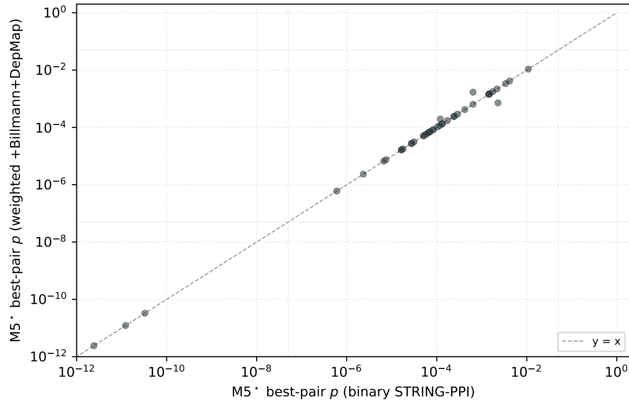
(A) Per-pair p_{\min} : binary vs weighted substrate
