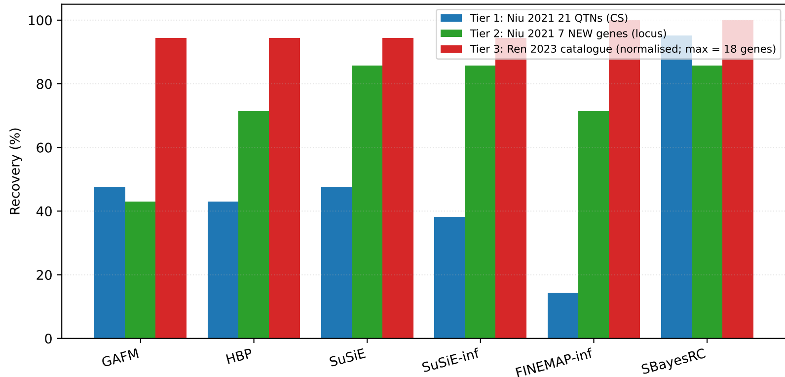
3kRG grain — fine-mapping recovery vs. Niu 2021 + Ren 2023 ground truth
