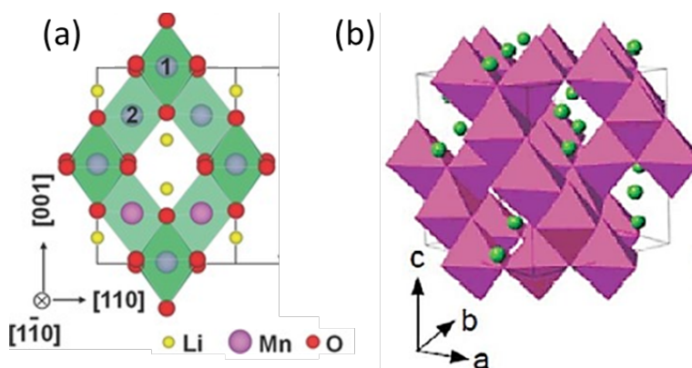
FIGURE 14 – Projection 2D de la structure \text{LiMn}_2\text{O}_4 (a) et structure 3D (b)
