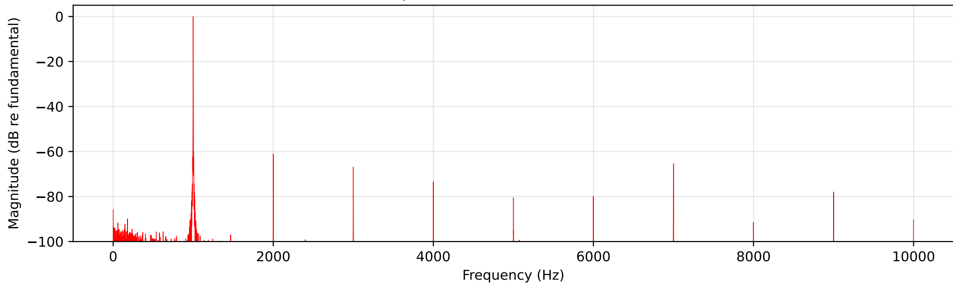
THD Spectrum (1 kHz, THD = 0.1162%)
