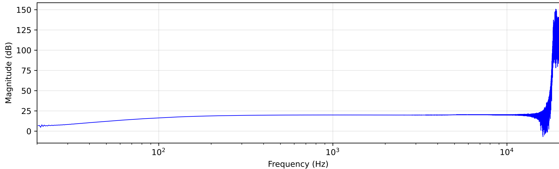
Frequency Response (loopback)
