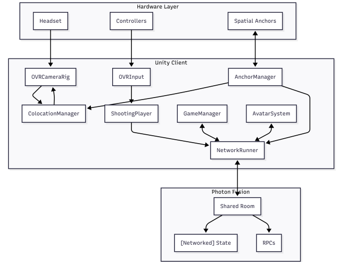
Fig. 1. System Architecture Diagram illustrating the data flow between Unity components, the networking layer, and the physical hardware layer.
