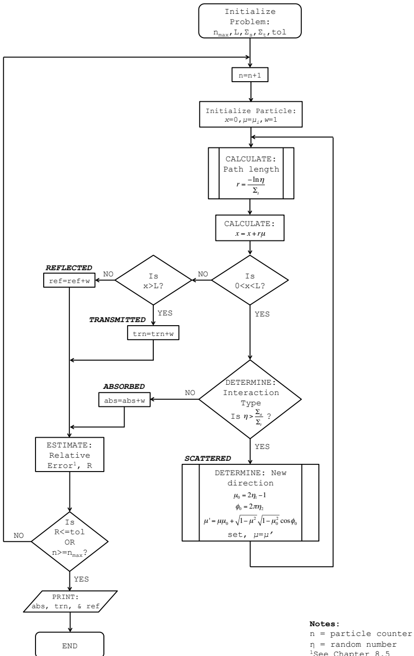
Figure 6.6 A flowchart for a Monte Carlo algorithm for simulation of a 1-D shield
