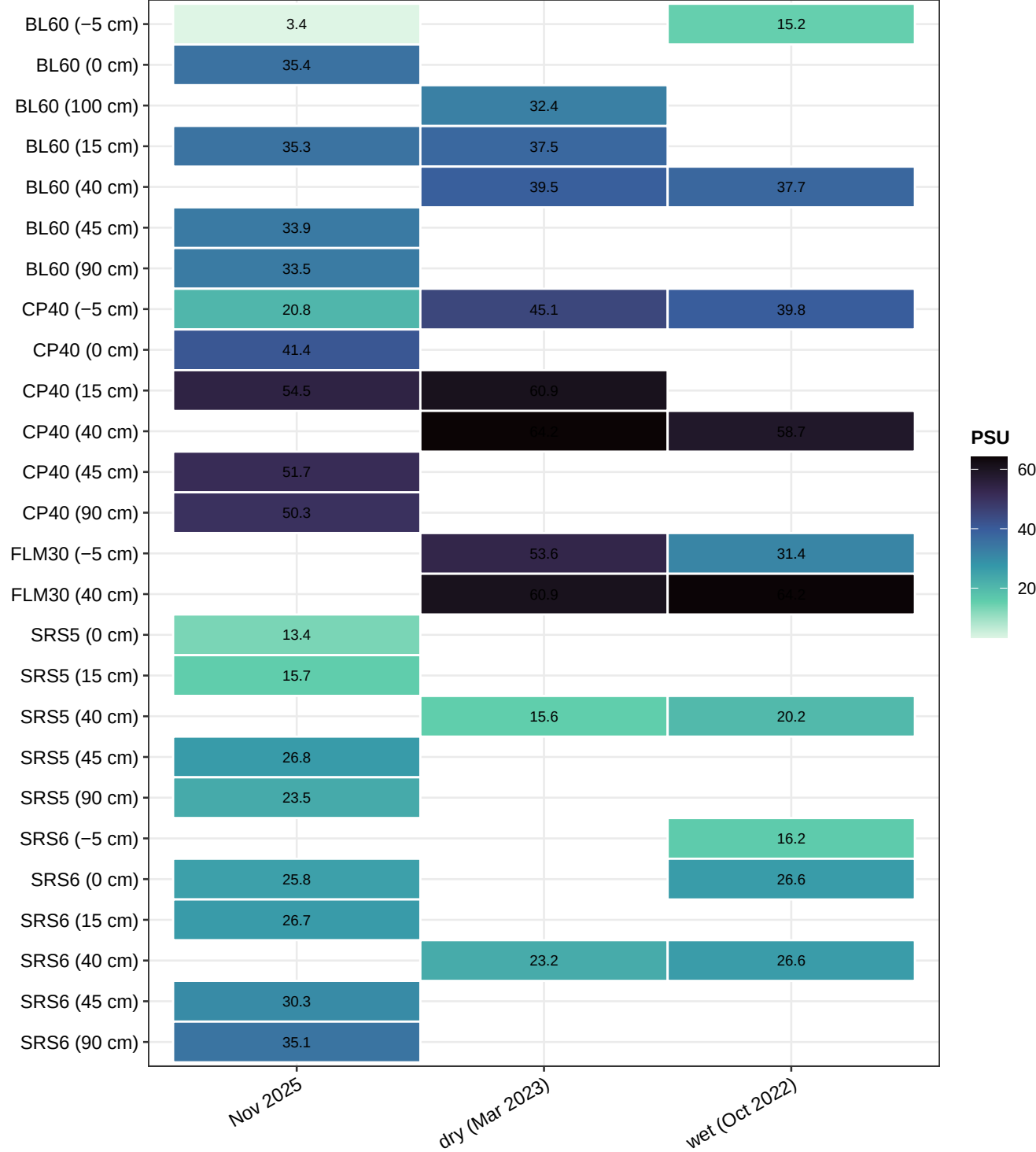
Salinity (PSU)
