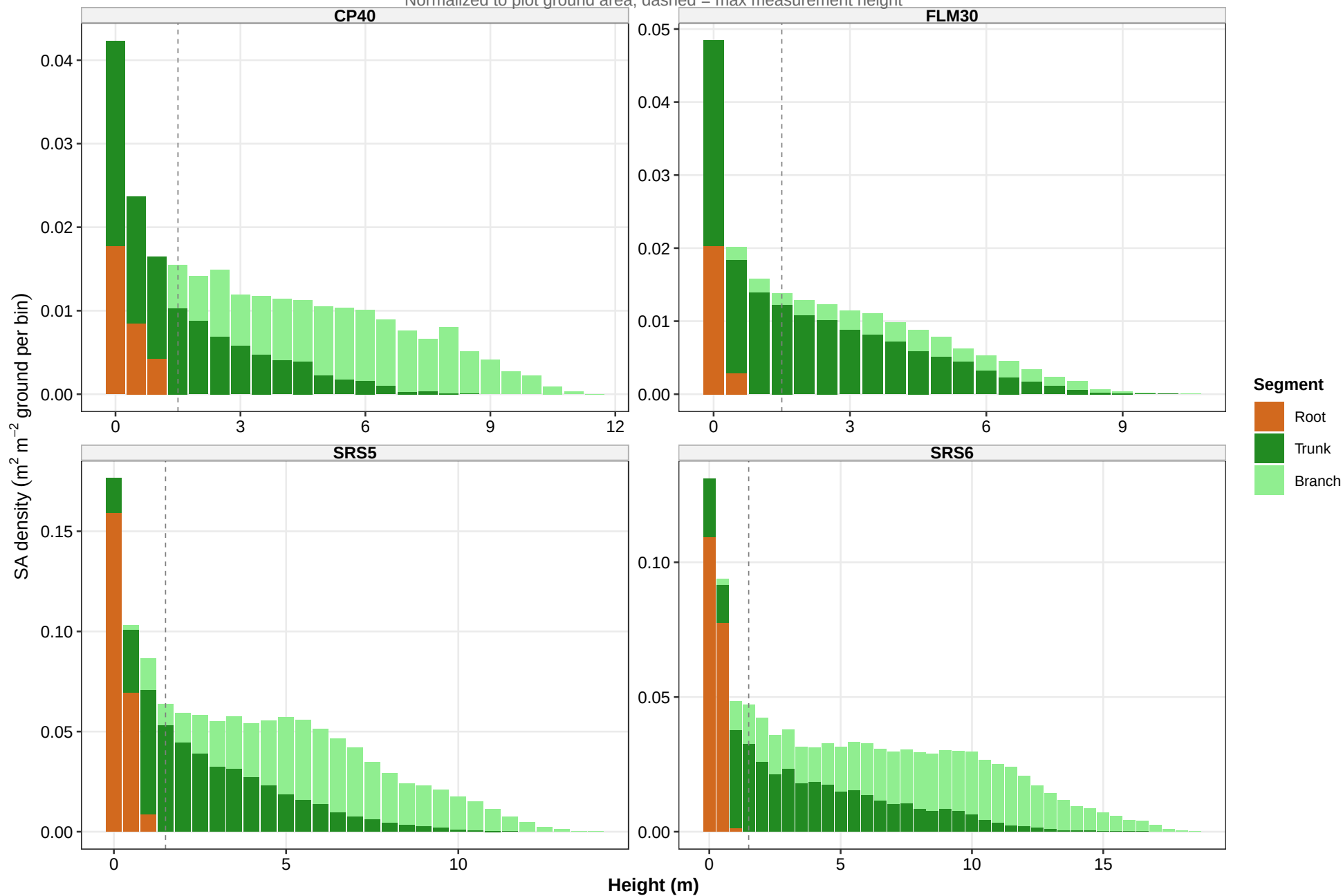
TLS surface area density profiles Normalized to plot ground area; dashed = max measurement height
