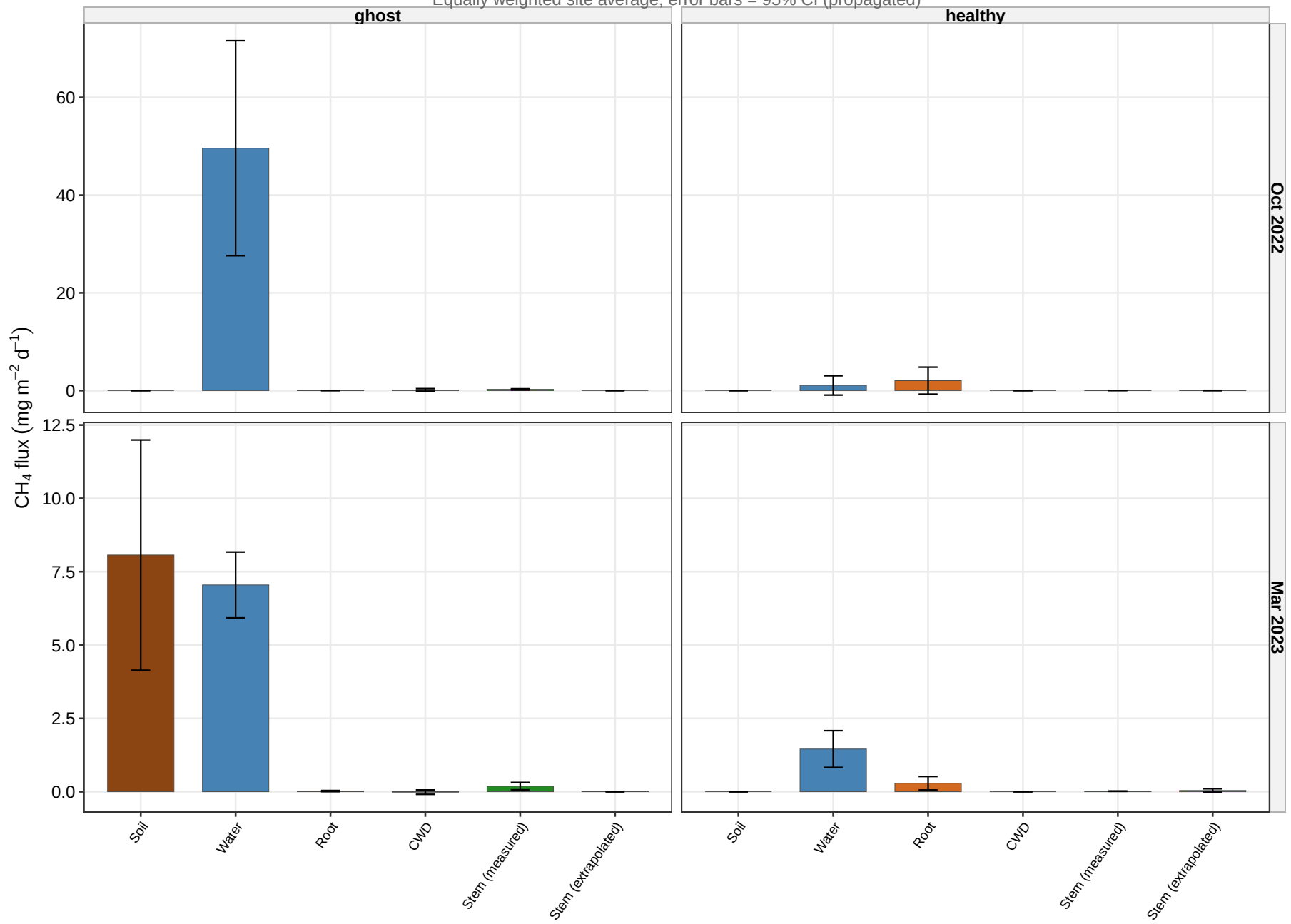
Disturbance-class mean CH 4 by component Equally weighted site average; error bars = 95% CI (propagated)
