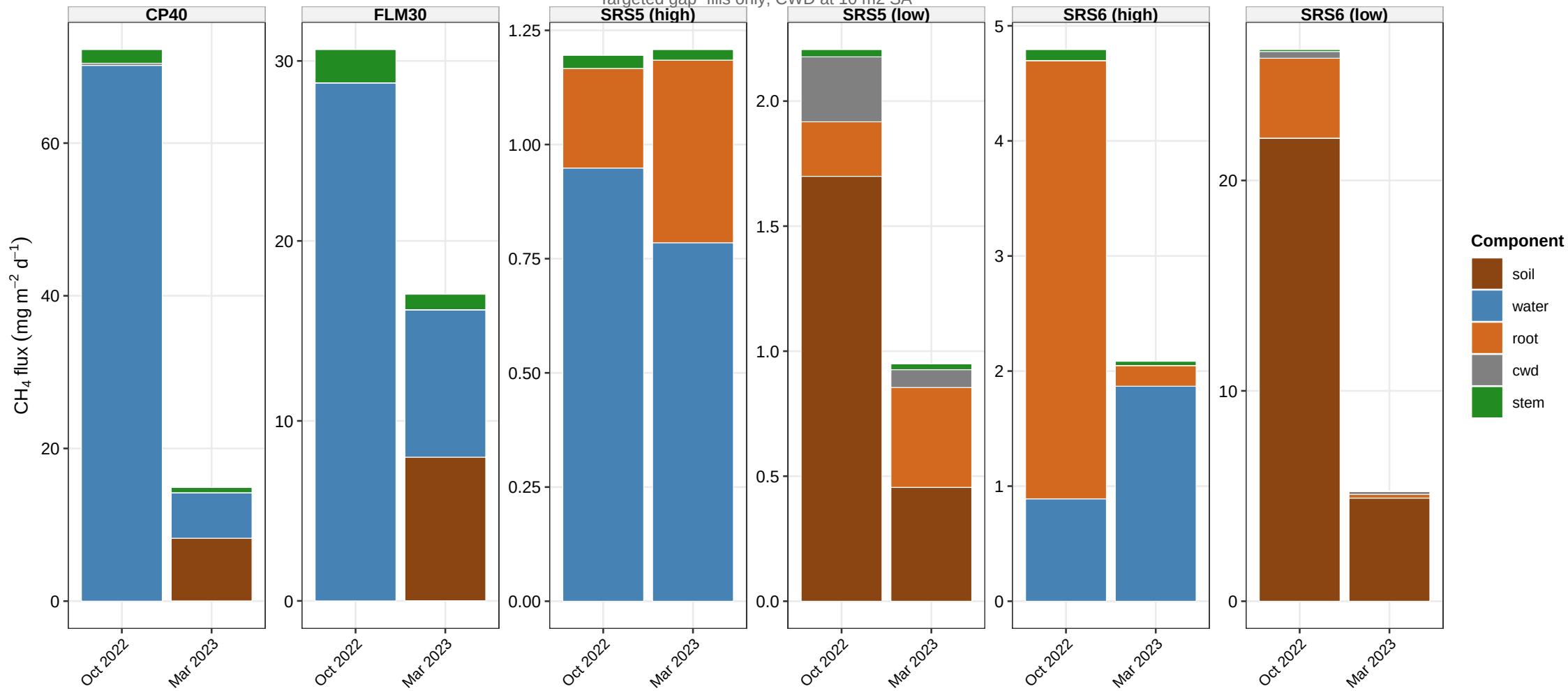
Plot-level CH 4 by component (zero above max)
