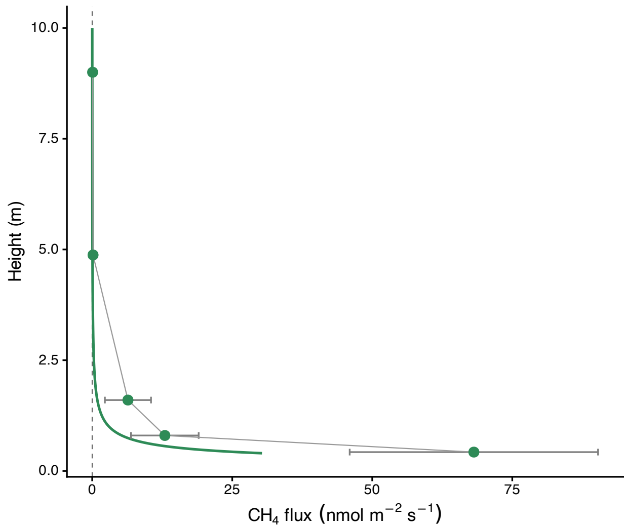
Mean CH 4 profile ( \pm SE), power-law fit flux = 3.0 \cdot h^{-2.5}
