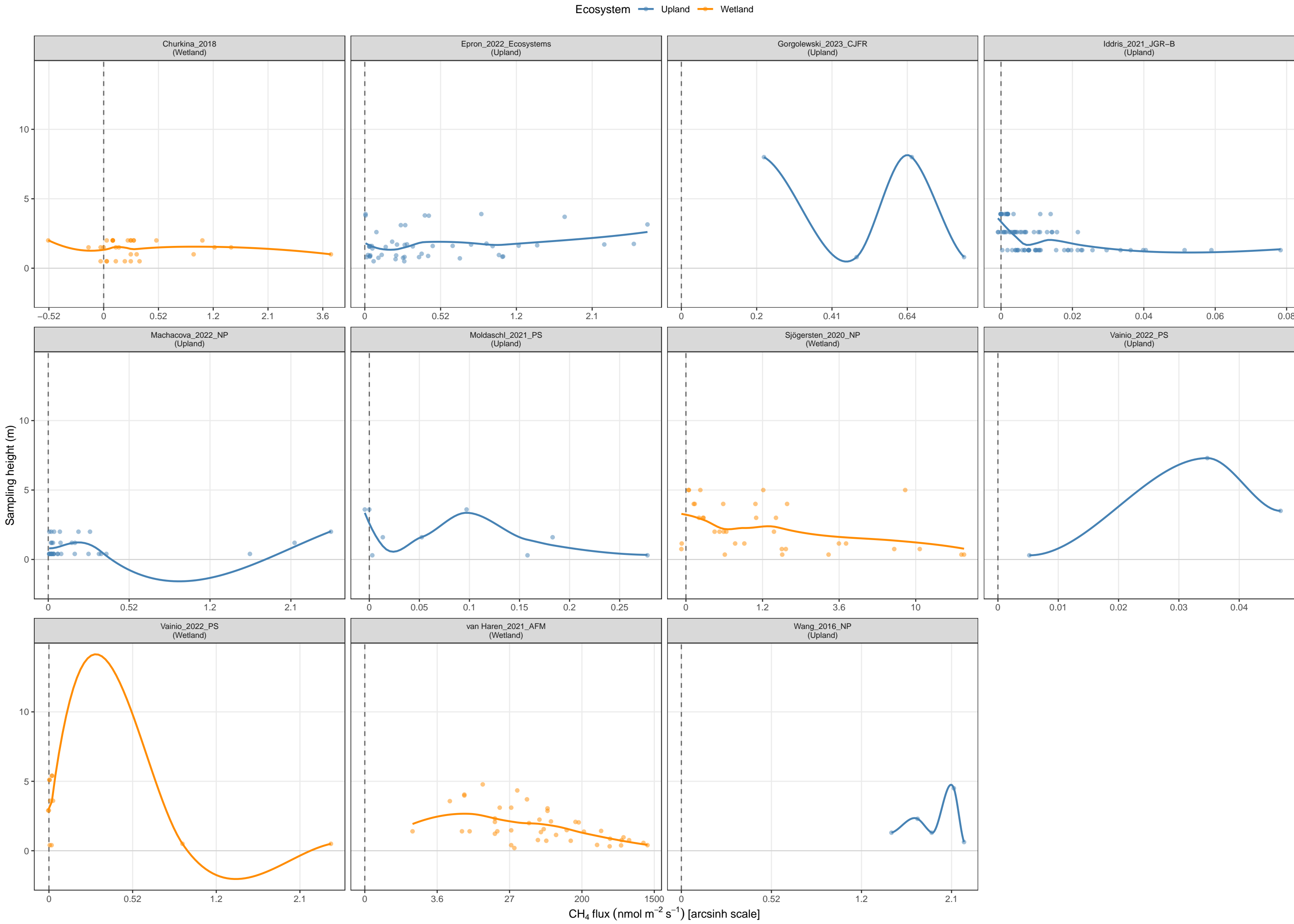
Stem CH 4 flux vs. height (projects with measurements >= 2 m) Free arcsinh-transformed flux axis
