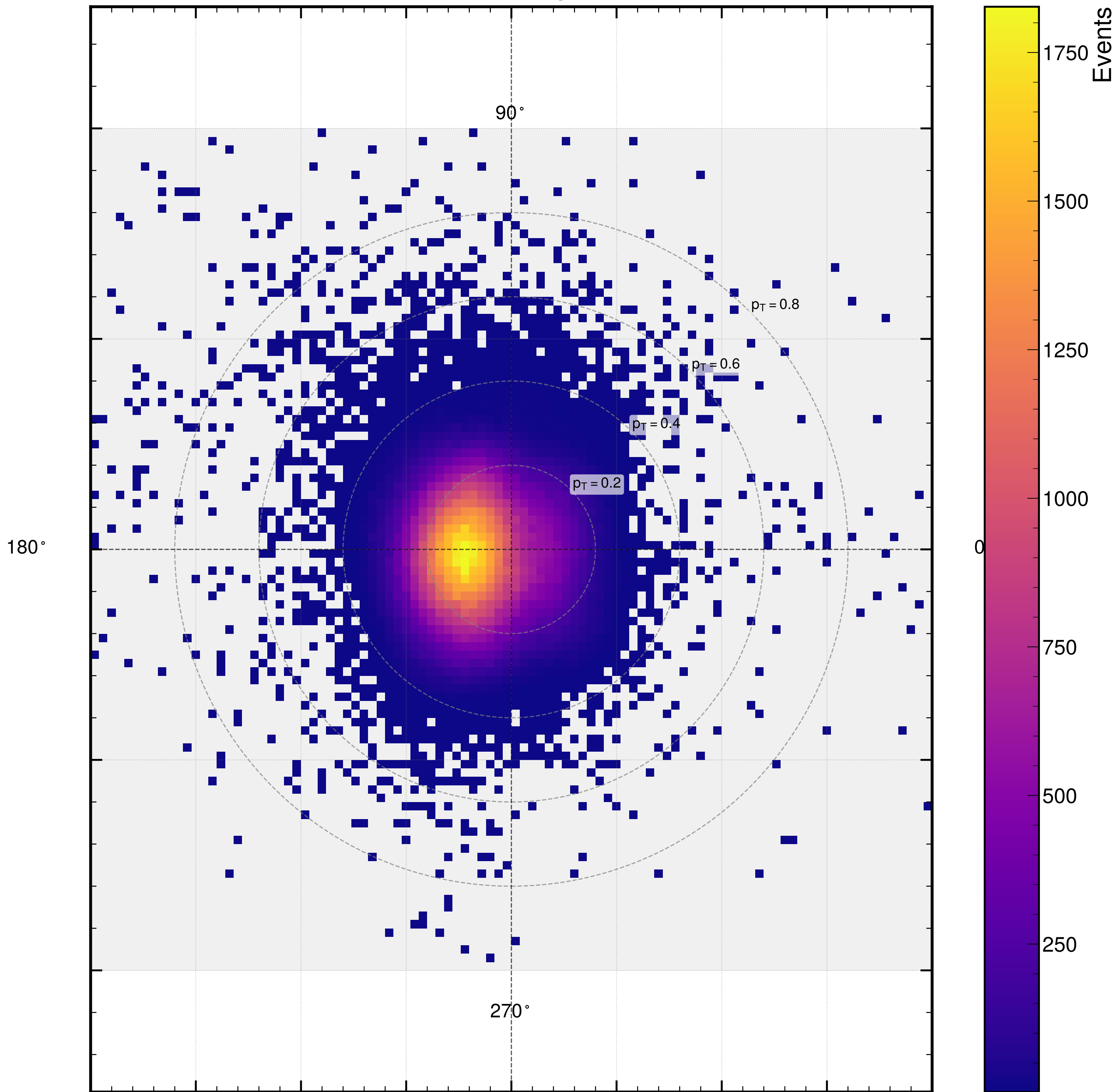
p_T vs \phi
