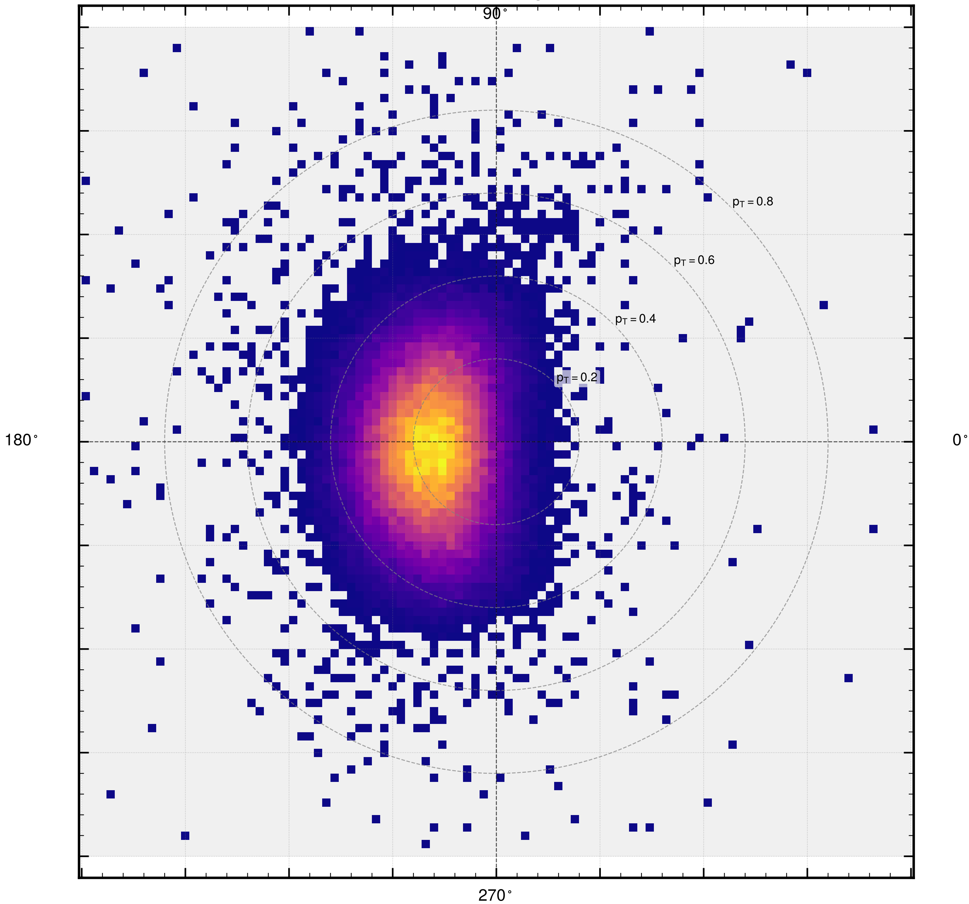
p_T vs \phi
