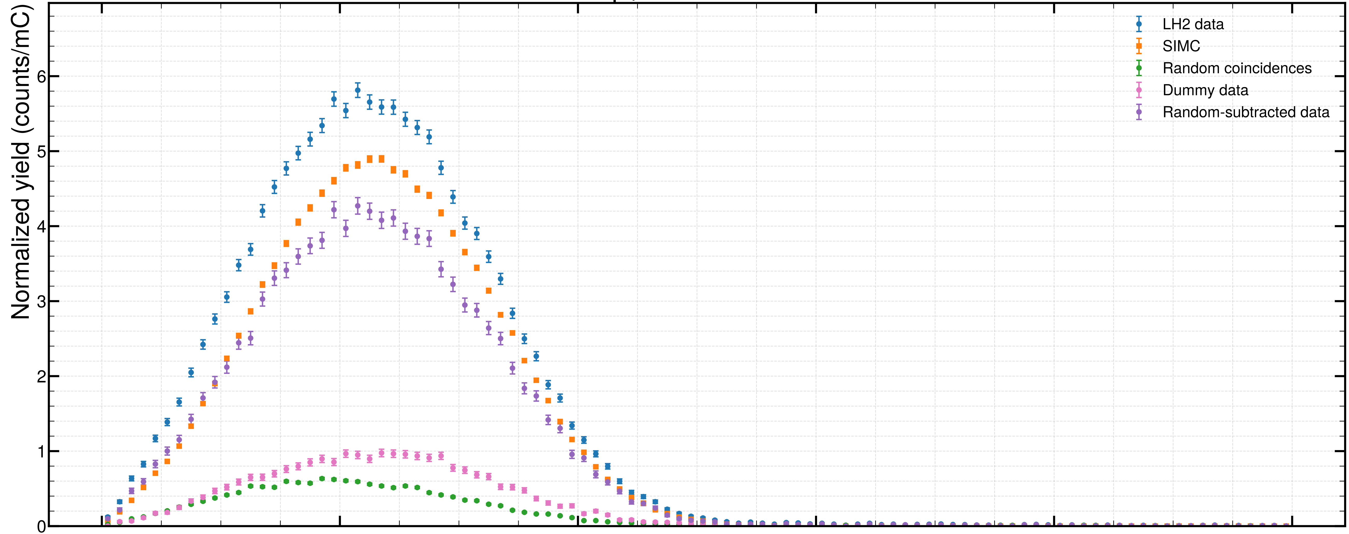
p_T distribution
