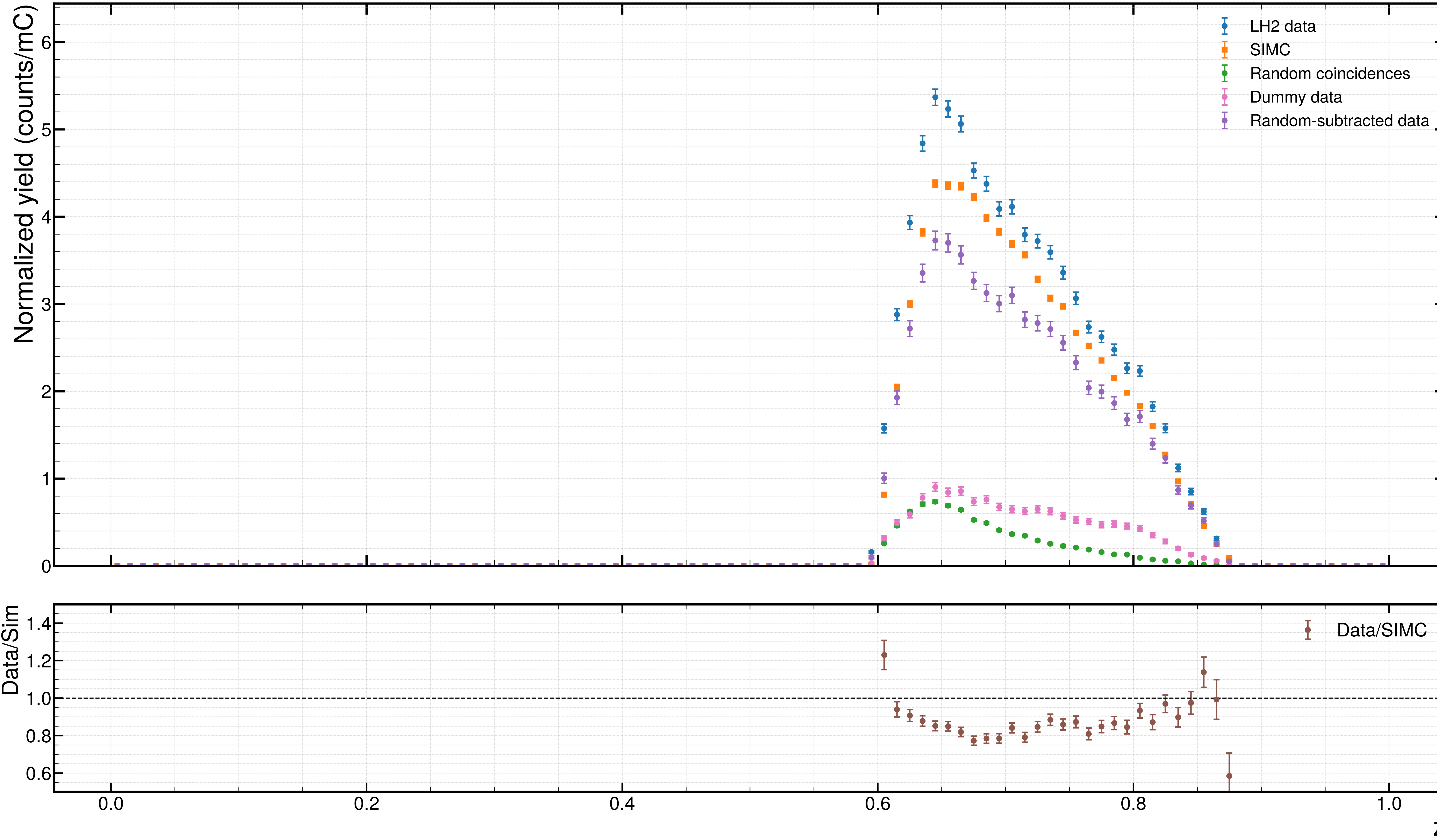
z distribution
