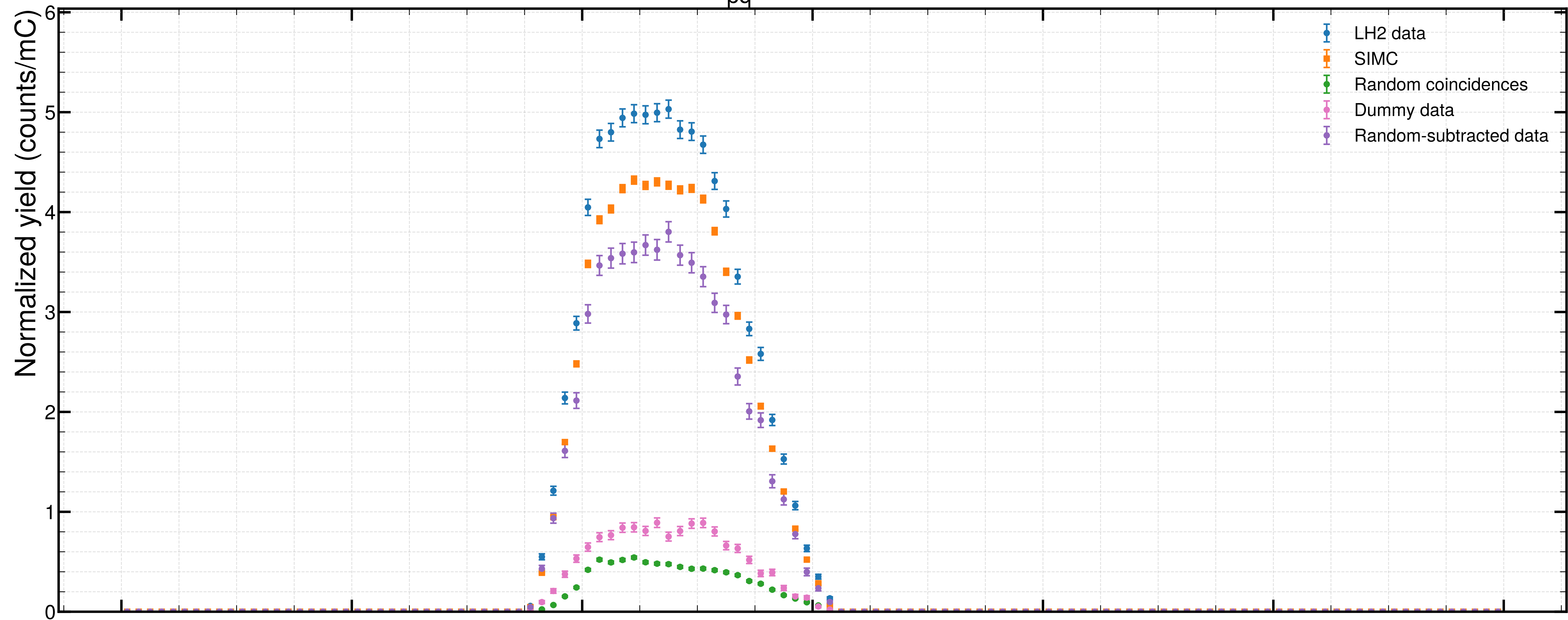
\theta_{pq} distribution
