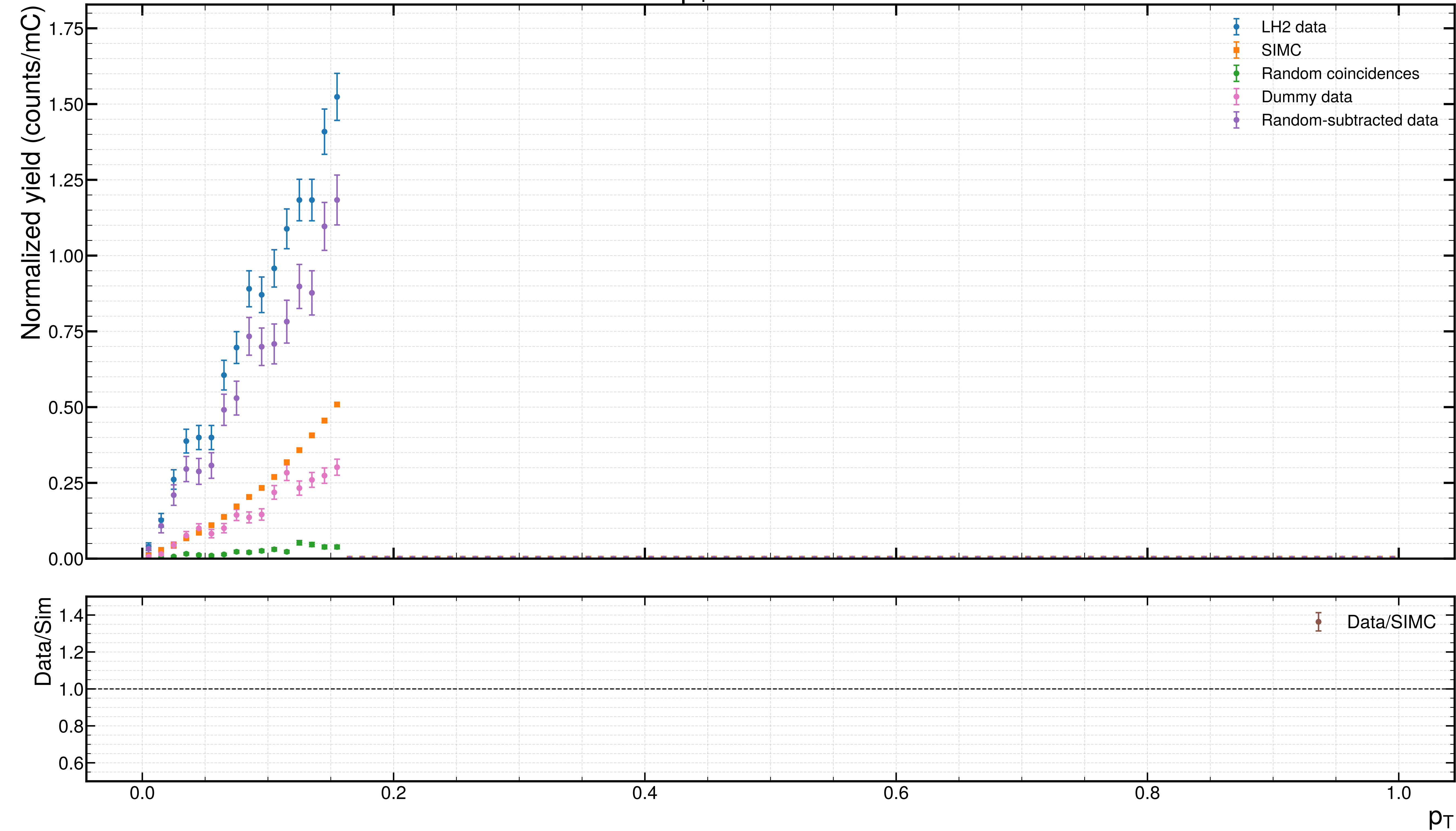
p_T distribution
