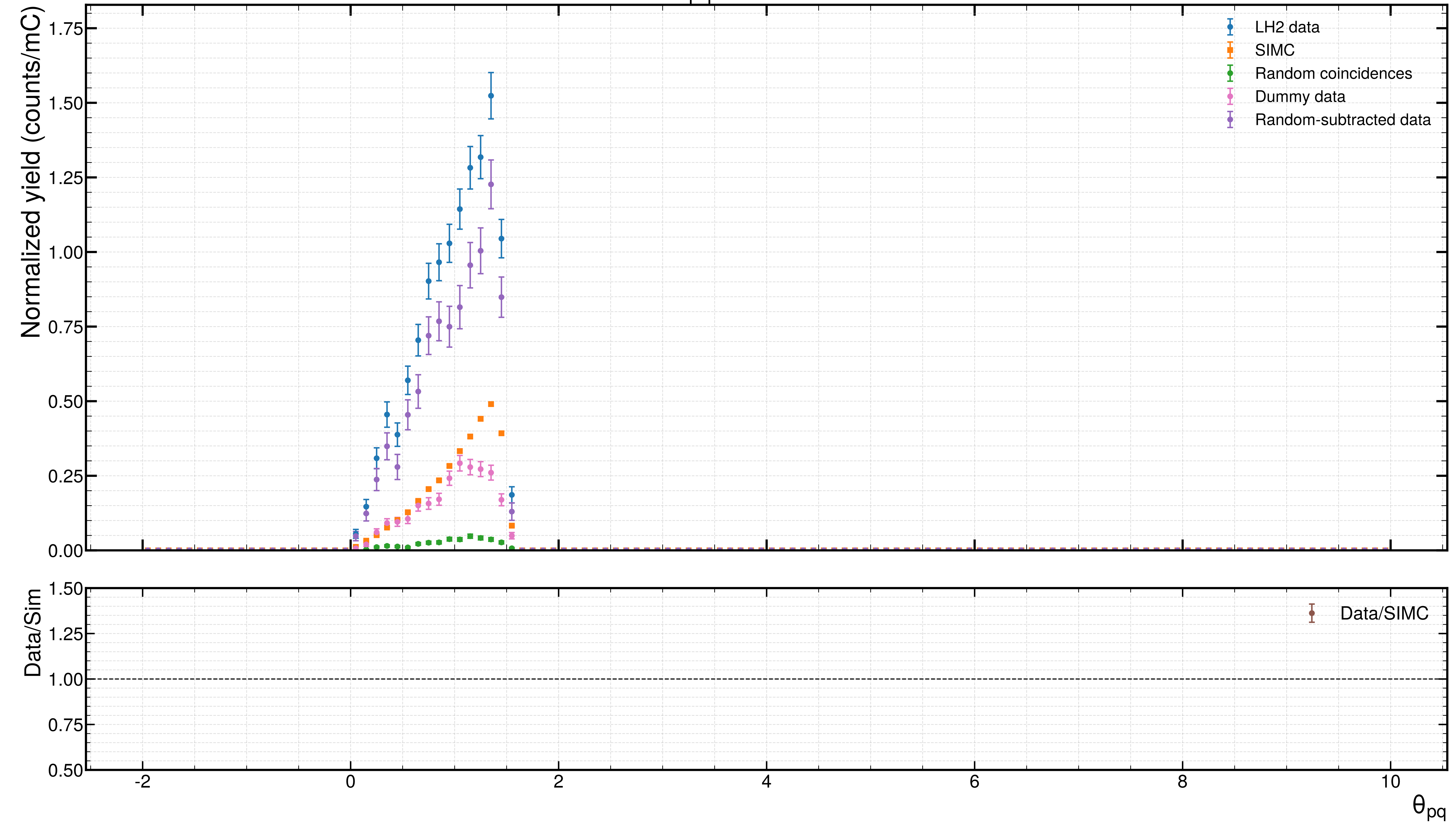
\theta_{pq} distribution
