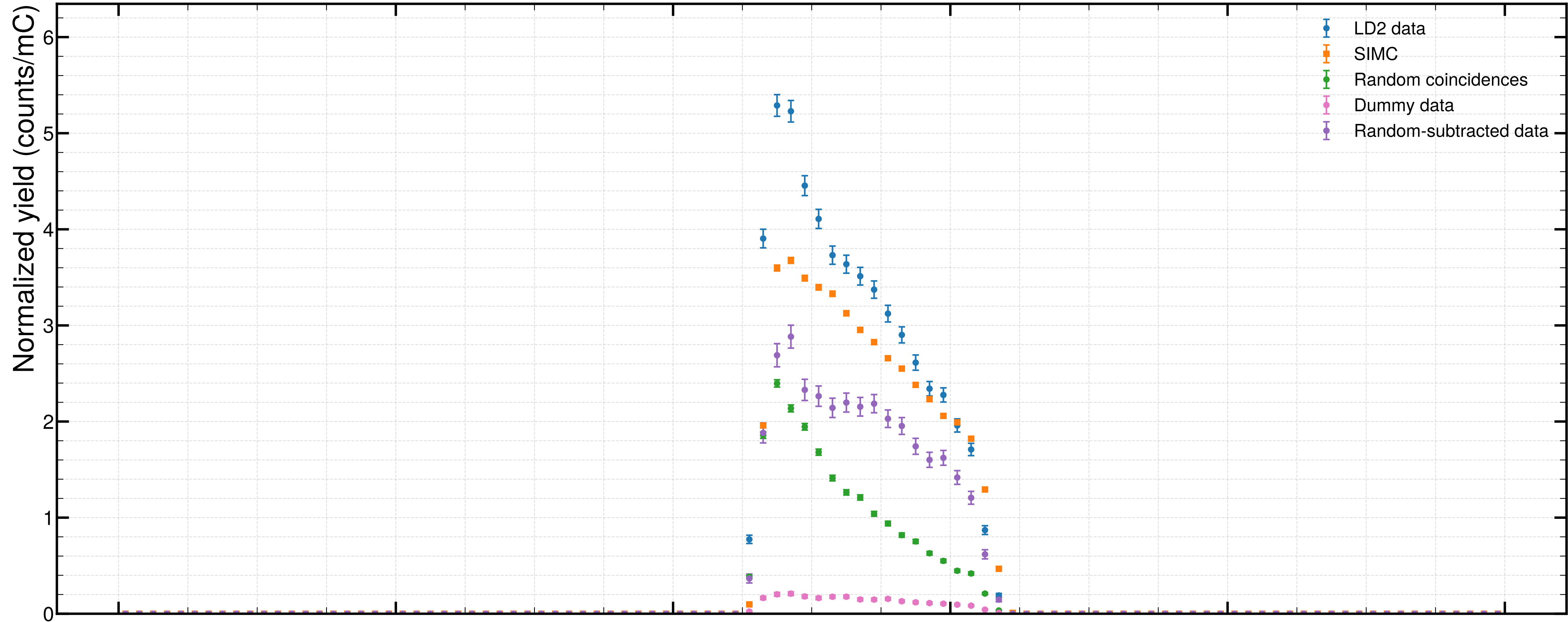
z distribution
