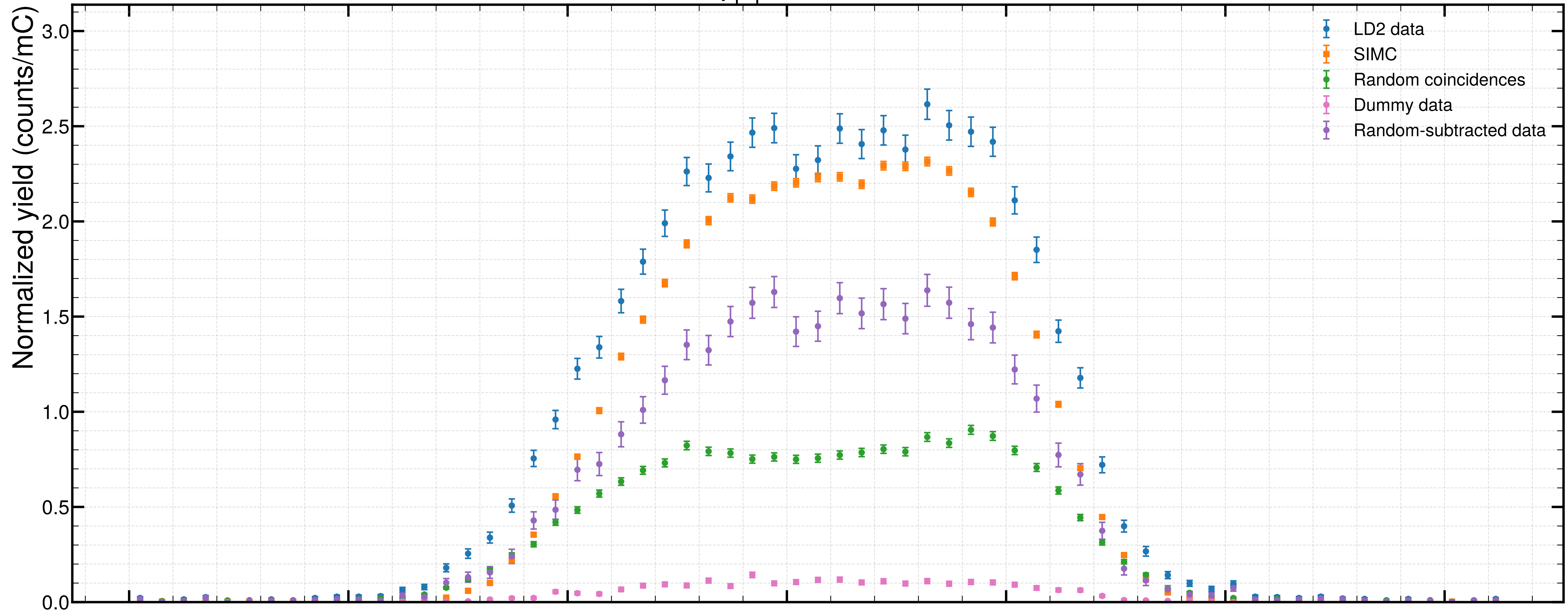
\phi_{pq} distribution
