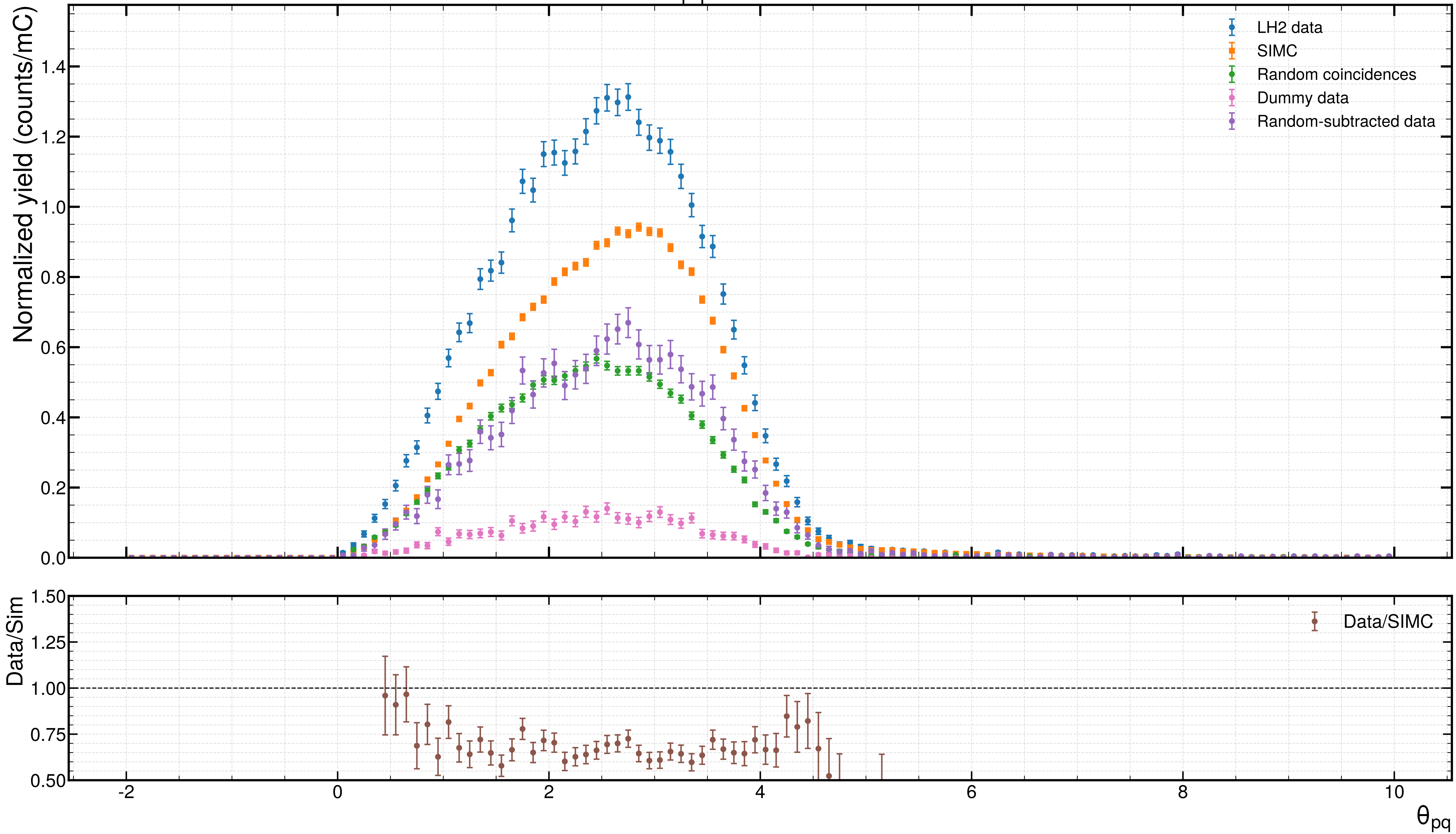
\theta_{pq} distribution
