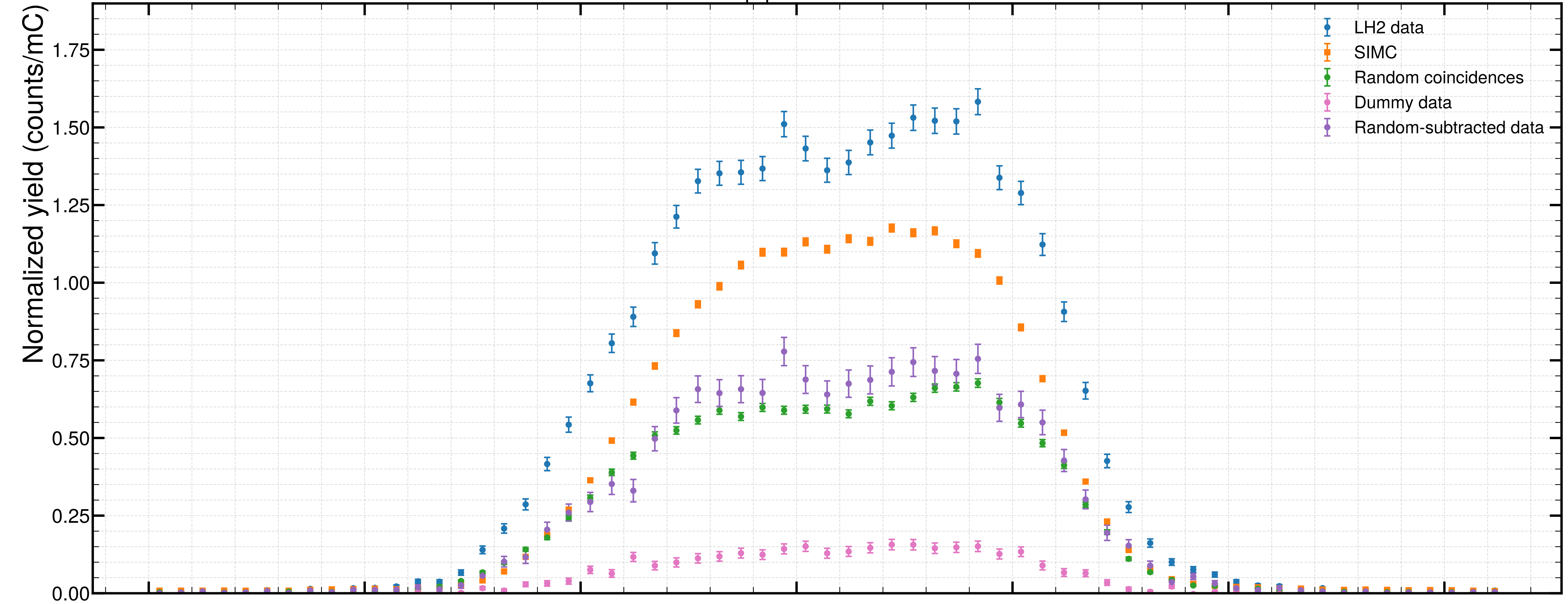
\phi_{pq} distribution
