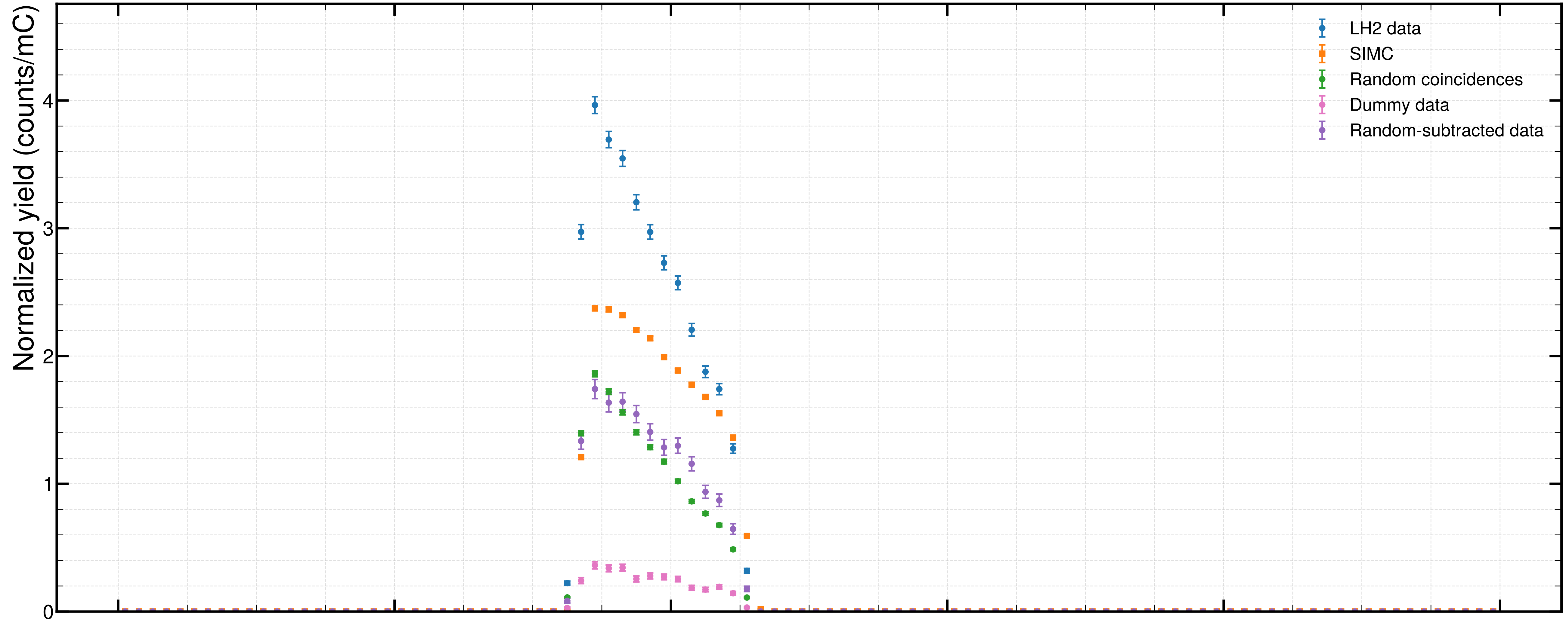
z distribution
