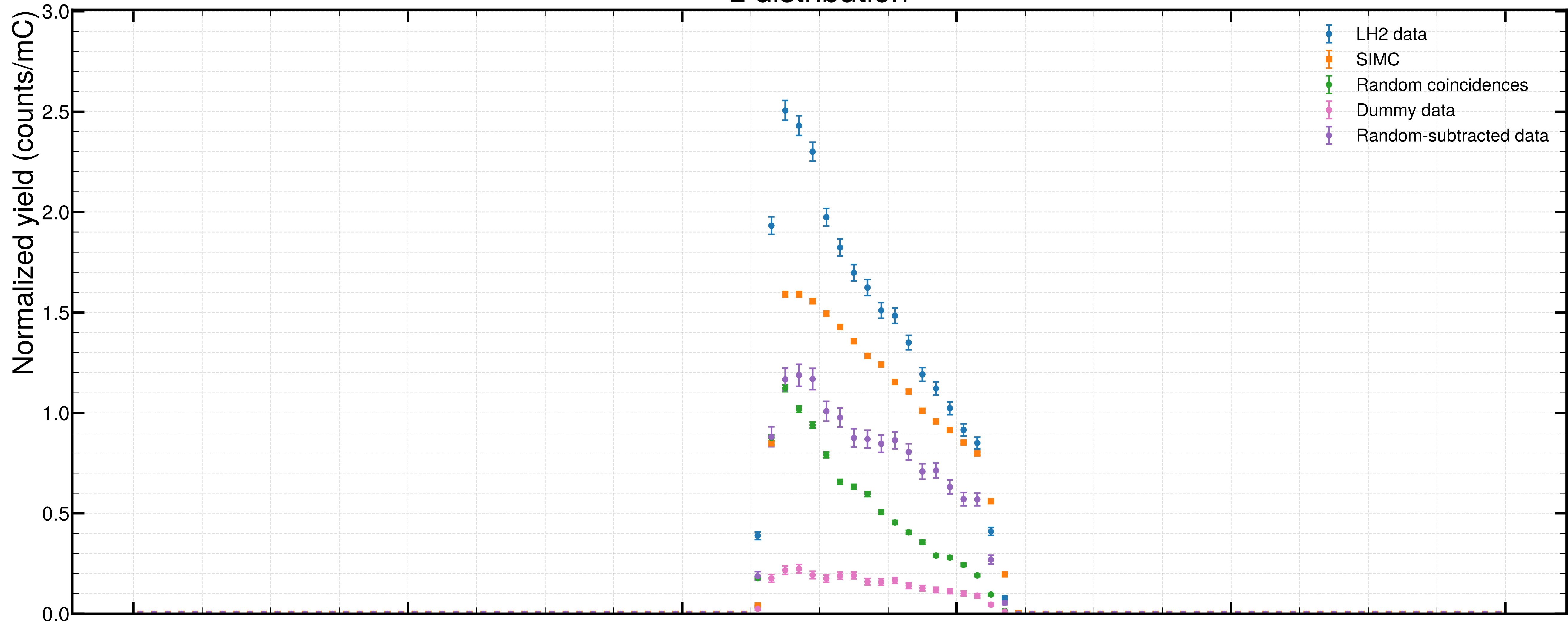
z distribution
