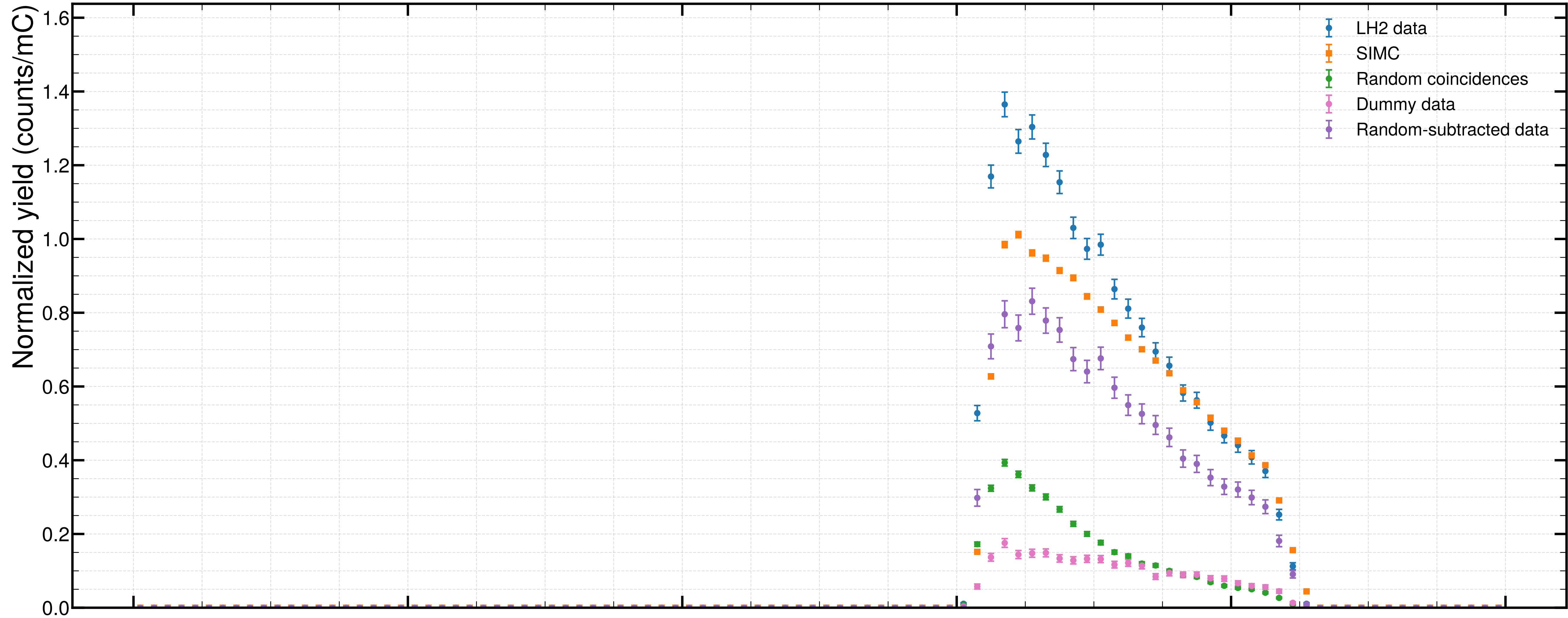
z distribution
