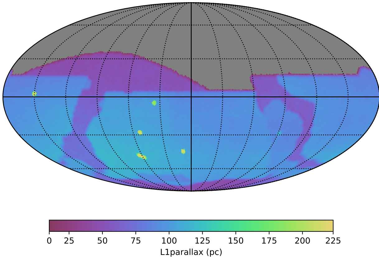
baseline_v5.0.0_10yrs : L1parallax
