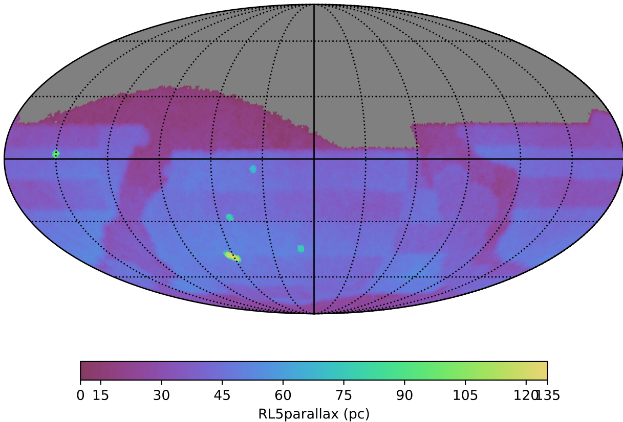
baseline_v5.0.0_10yrs night < 730: RL5parallax
