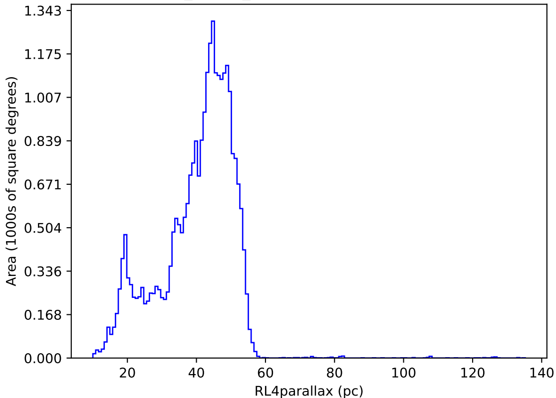
baseline_v5.0.0_10yrs night < 730: RL4parallax
