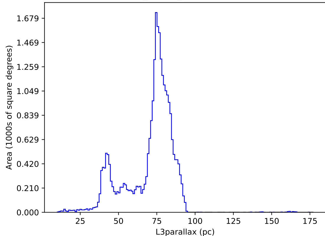
baseline_v5.0.0_10yrs : L3parallax
