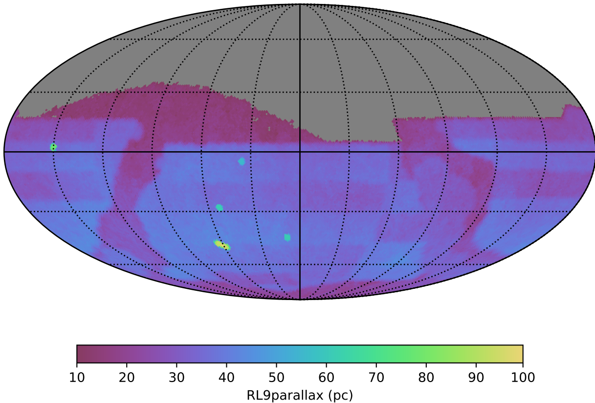
baseline_v5.0.0_10yrs night < 730: RL9parallax
