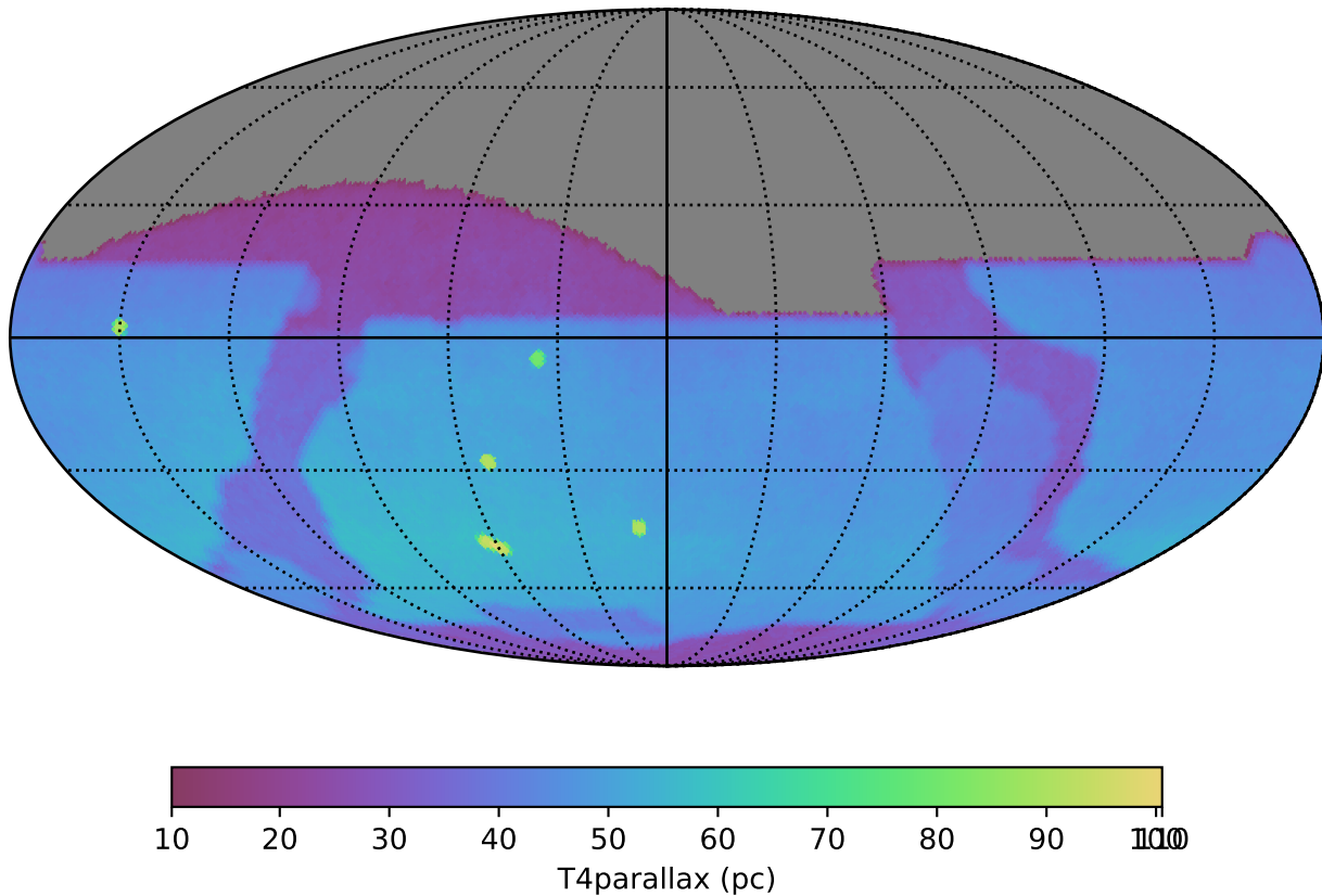
baseline_v5.0.0_10yrs : T4parallax
