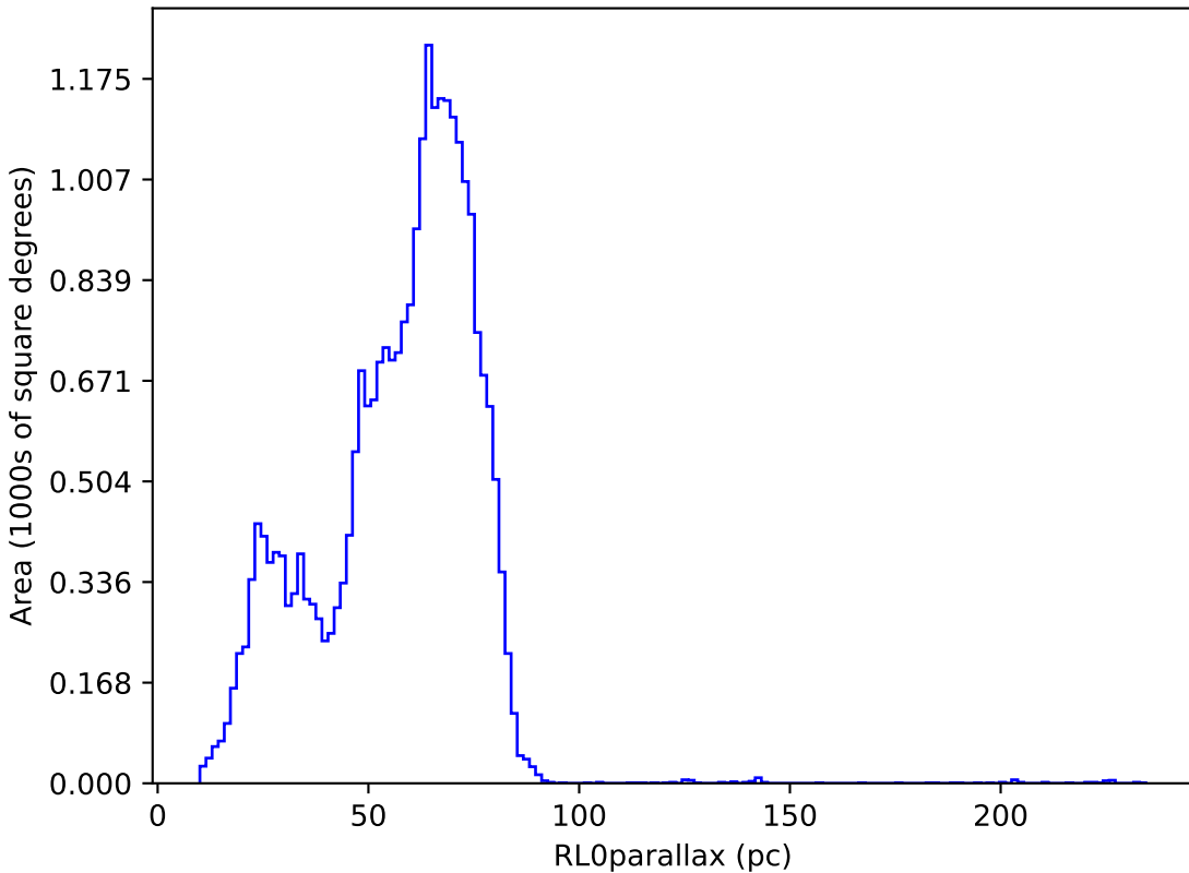
baseline_v5.0.0_10yrs night < 730: RL0parallax
