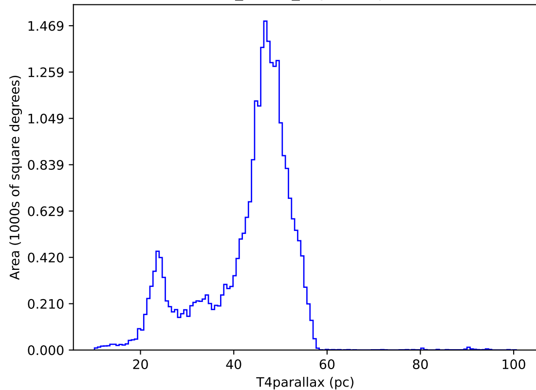
baseline_v5.0.0_10yrs : T4parallax
