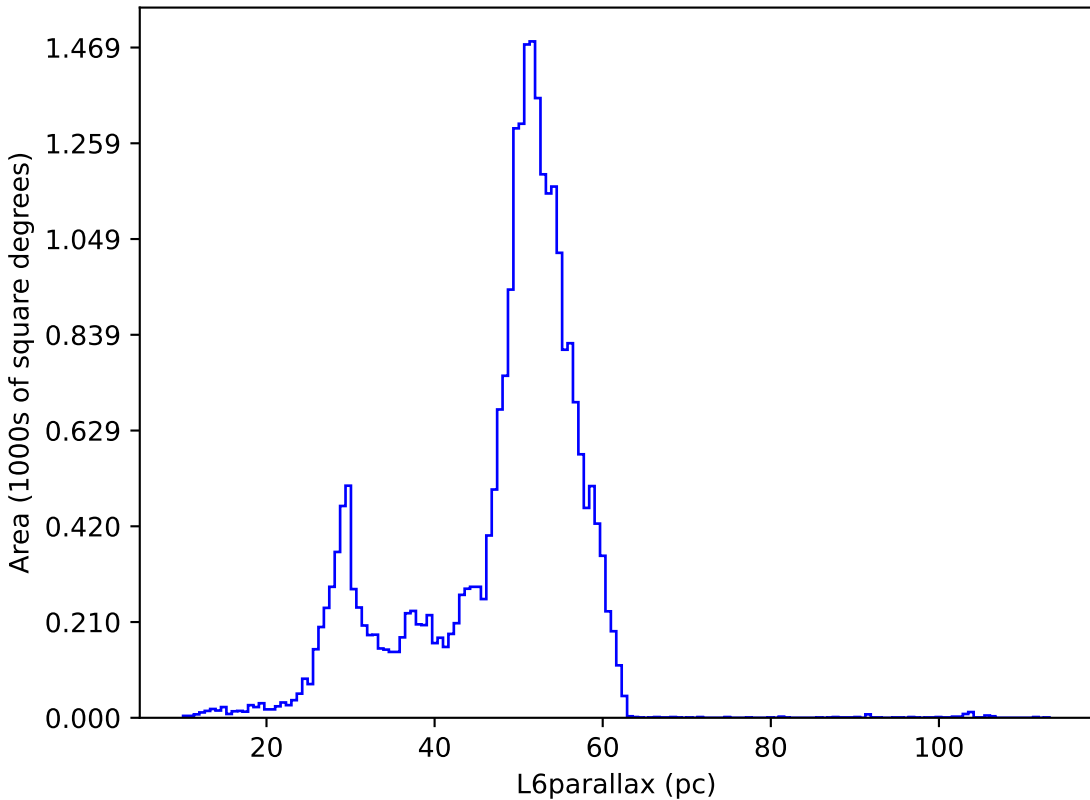
baseline_v5.0.0_10yrs : L6parallax
