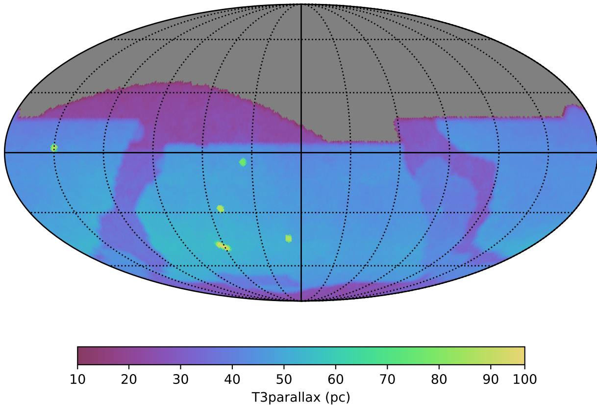
baseline_v5.0.0_10yrs : T3parallax
