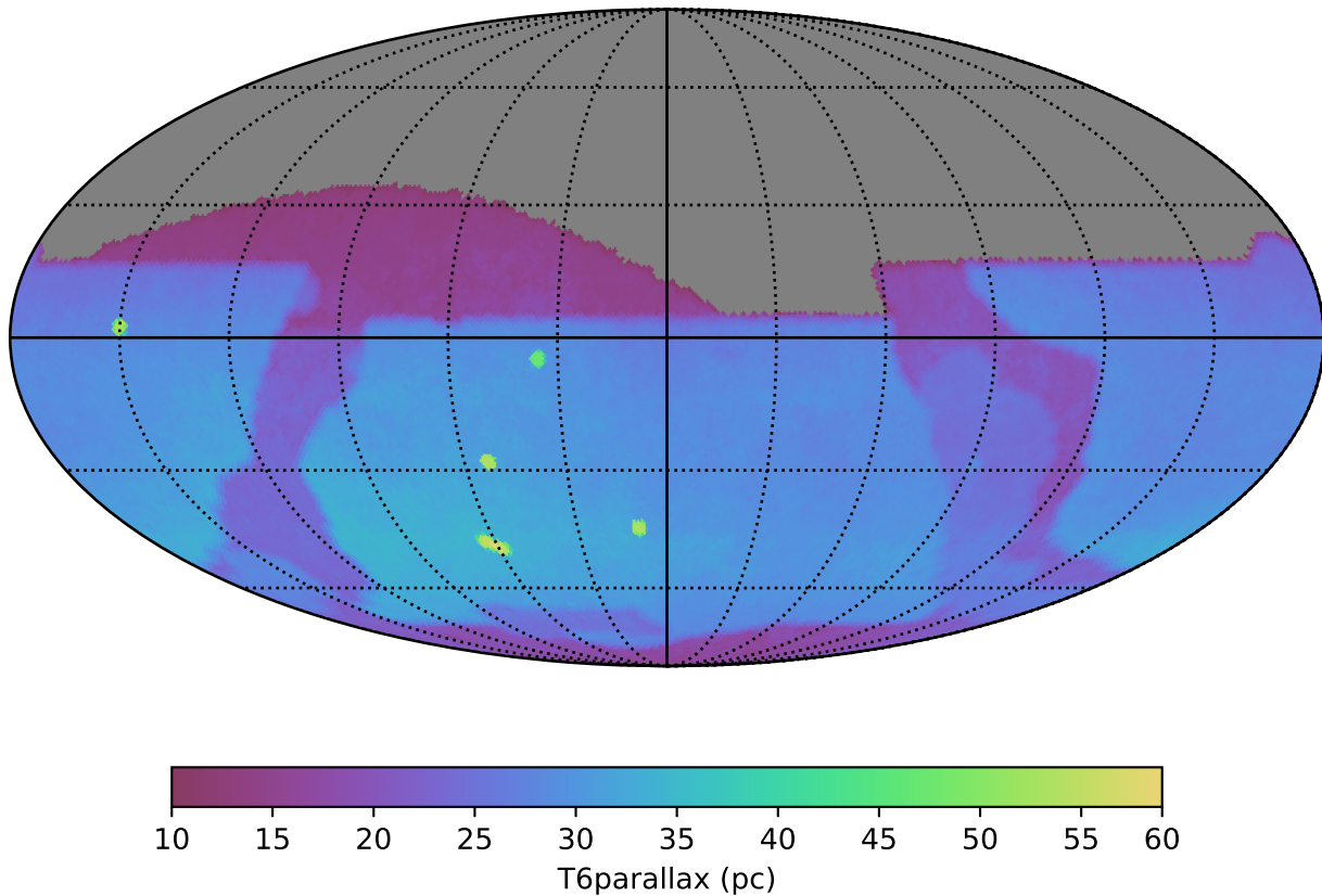
baseline_v5.0.0_10yrs : T6parallax
