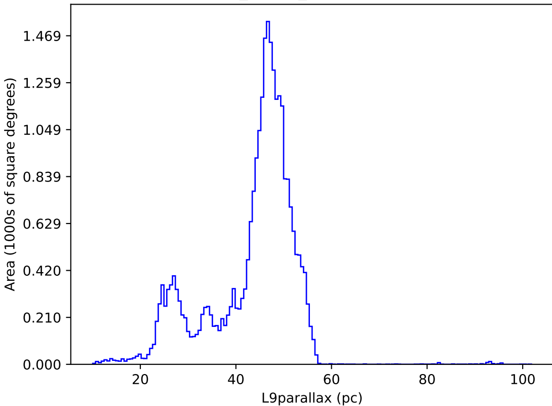
baseline_v5.0.0_10yrs : L9parallax
