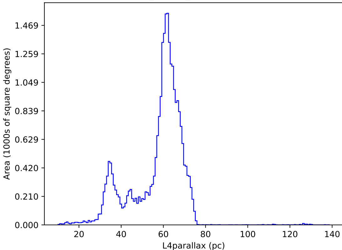
baseline_v5.0.0_10yrs : L4parallax
