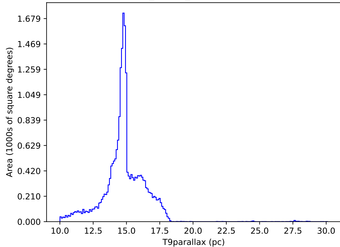
baseline_v5.0.0_10yrs : T9parallax
