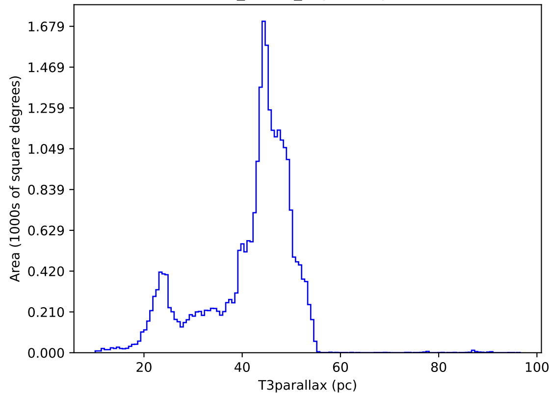
baseline_v5.0.0_10yrs : T3parallax
