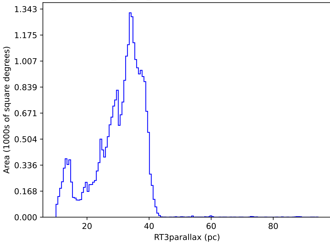
baseline_v5.0.0_10yrs night < 730: RT3parallax
