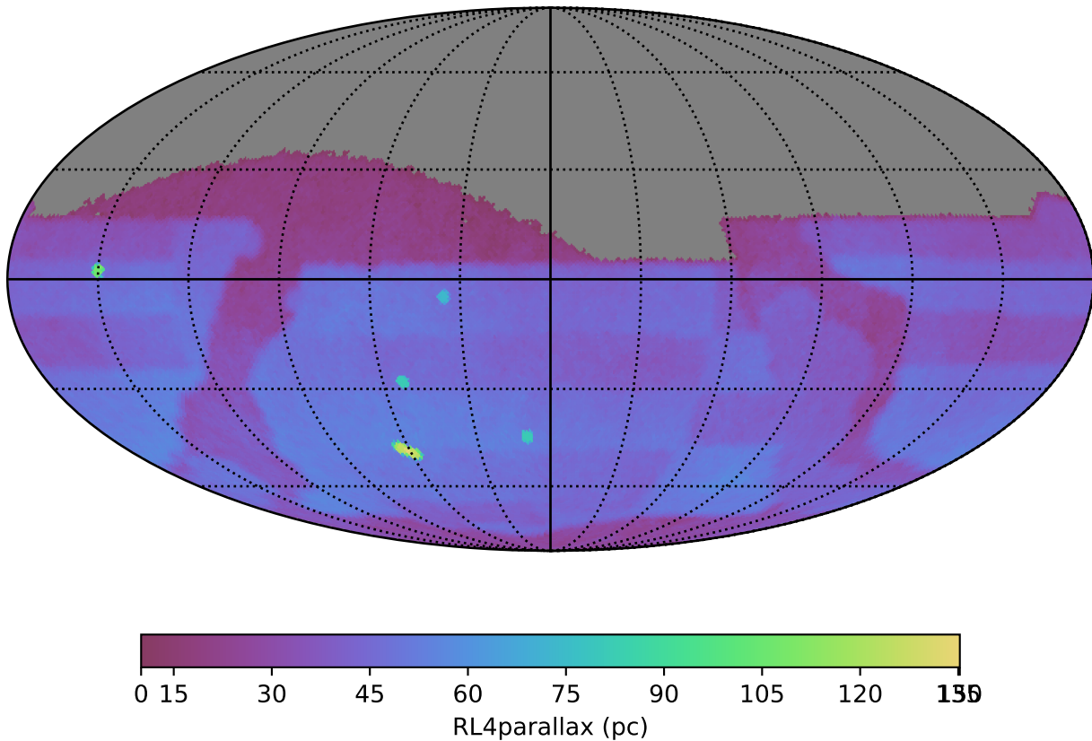
baseline_v5.0.0_10yrs night < 730: RL4parallax
