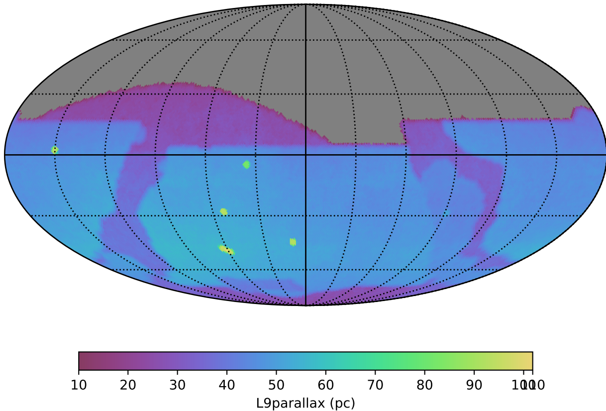
baseline_v5.0.0_10yrs : L9parallax
