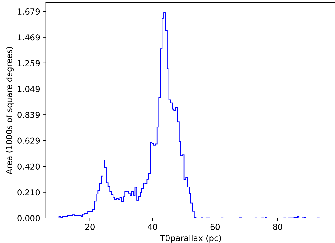
baseline_v5.0.0_10yrs : T0parallax
