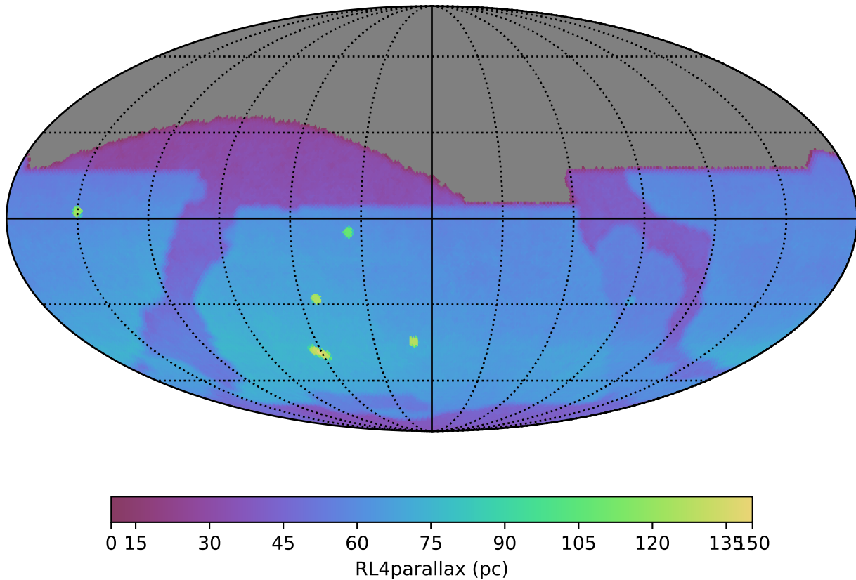
baseline_production_v5.0.1_10yrs : RL4parallax
