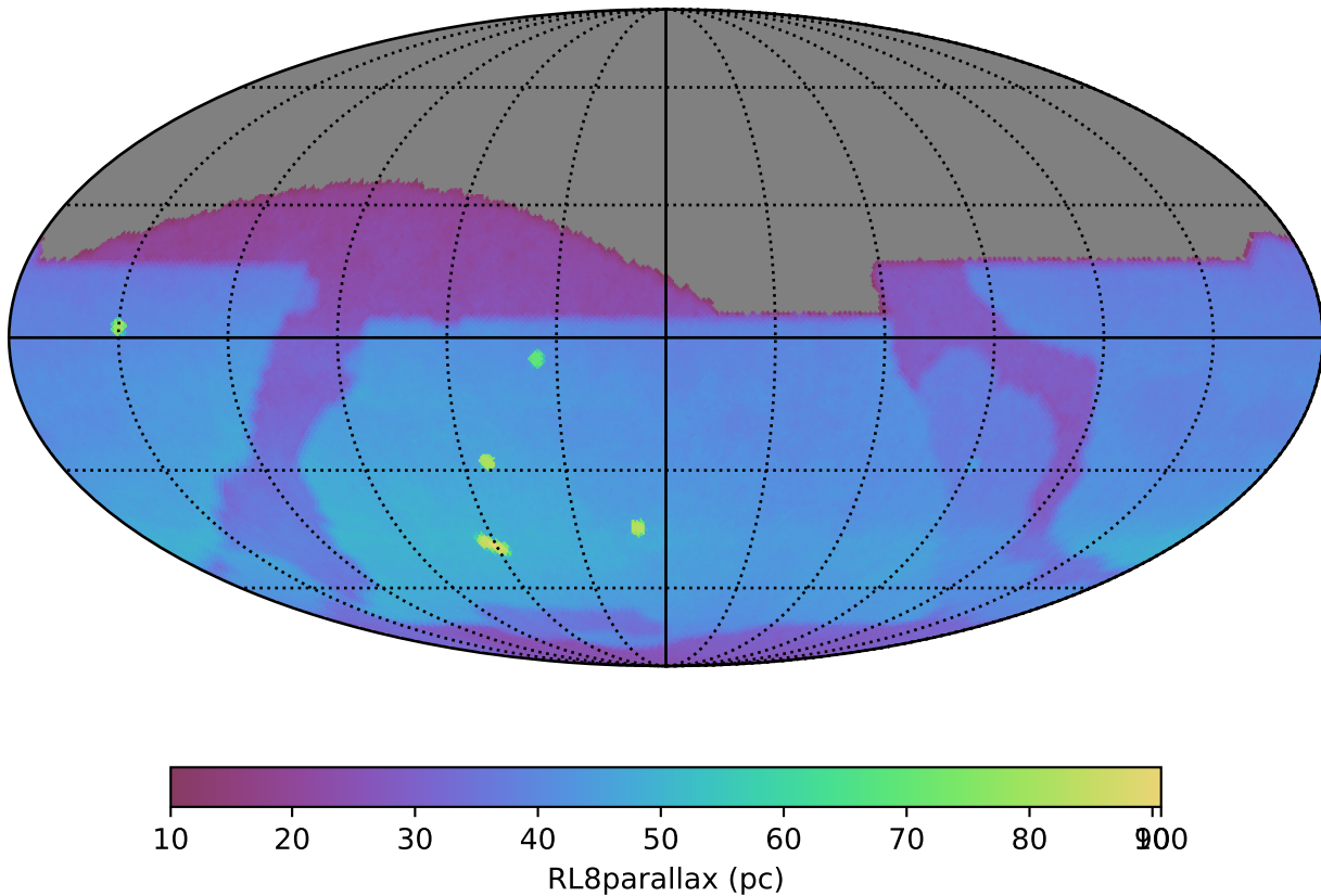
baseline_production_v5.0.1_10yrs : RL8parallax
