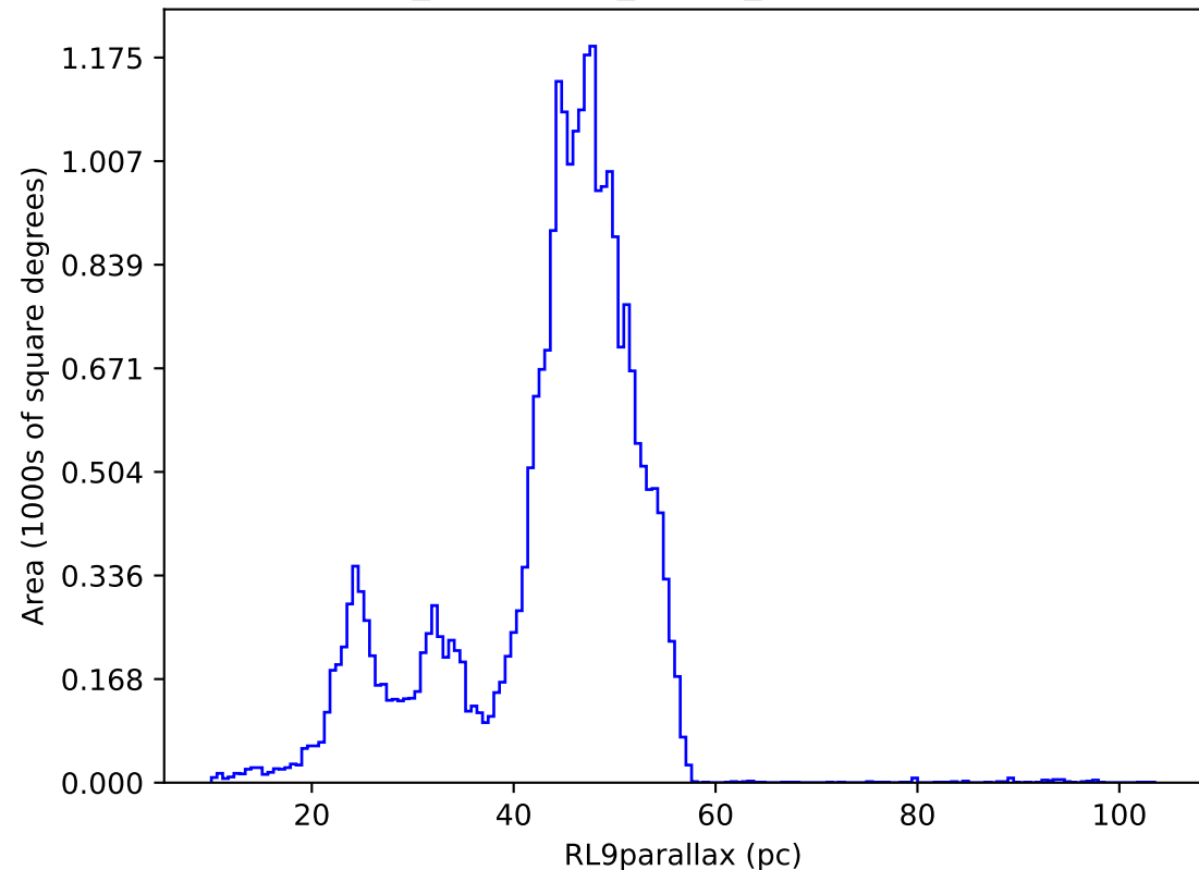
baseline_production_v5.0.1_10yrs : RL9parallax
