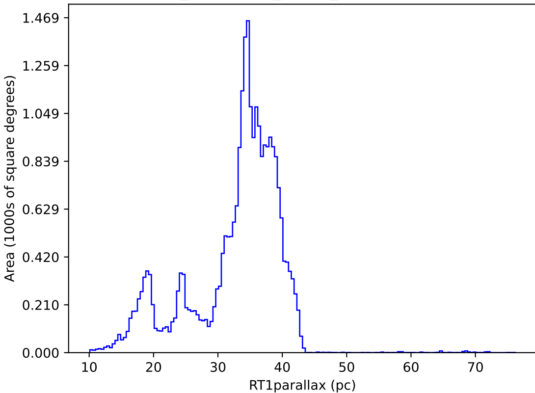
baseline_production_v5.0.1_10yrs : RT1parallax
