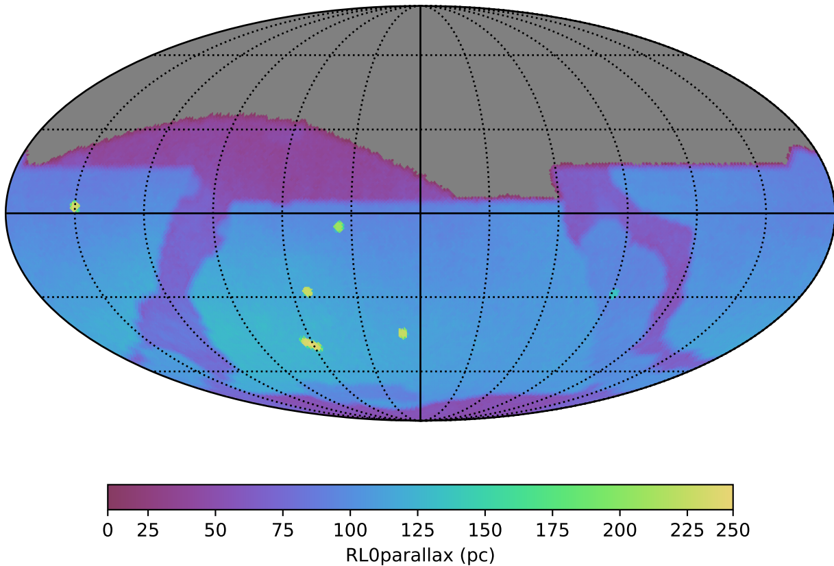
baseline_v5.3.0_10yrs : RL0parallax
