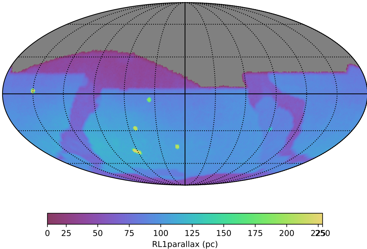
baseline_v5.3.0_10yrs : RL1parallax
