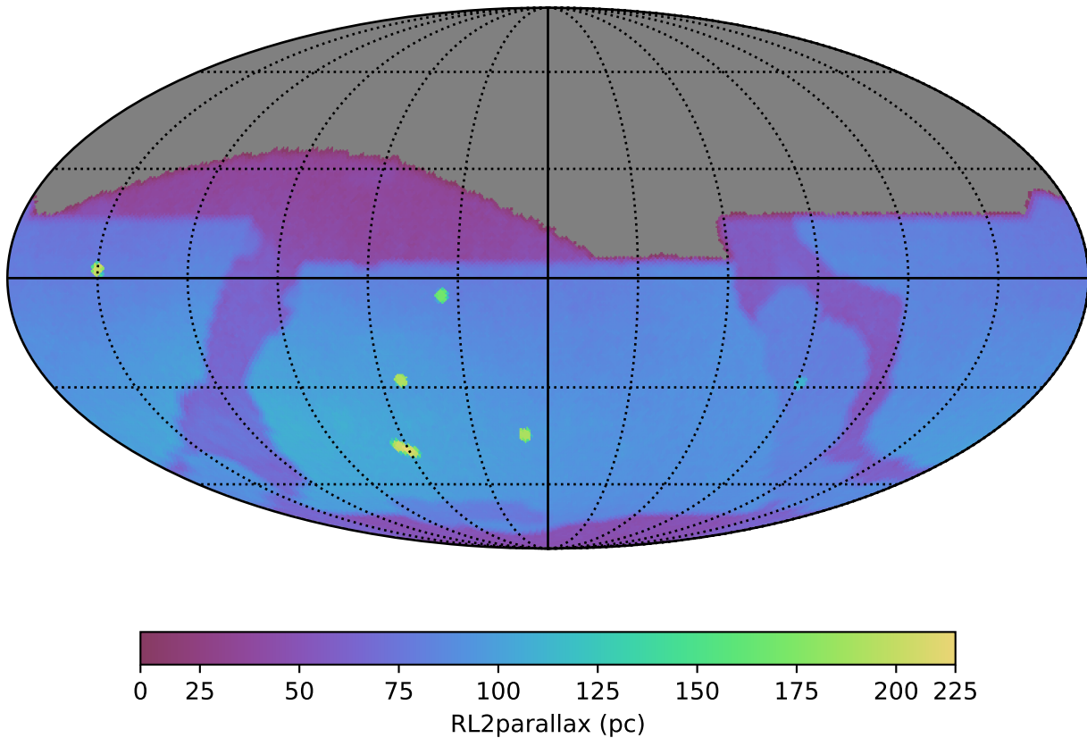
baseline_v5.3.0_10yrs : RL2parallax
