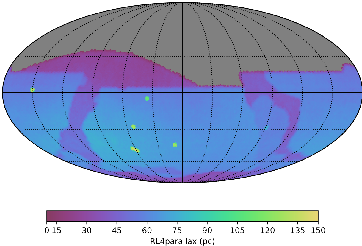
baseline_v5.3.0_10yrs : RL4parallax
