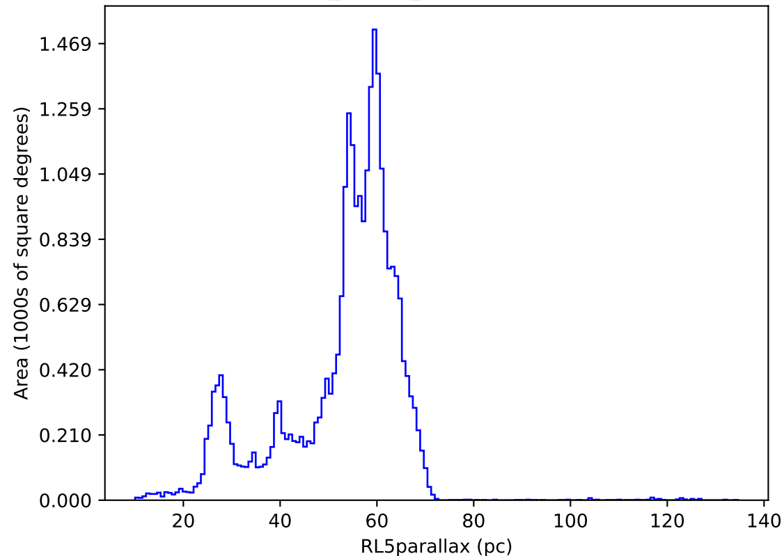
baseline_v5.3.0_10yrs : RL5parallax
