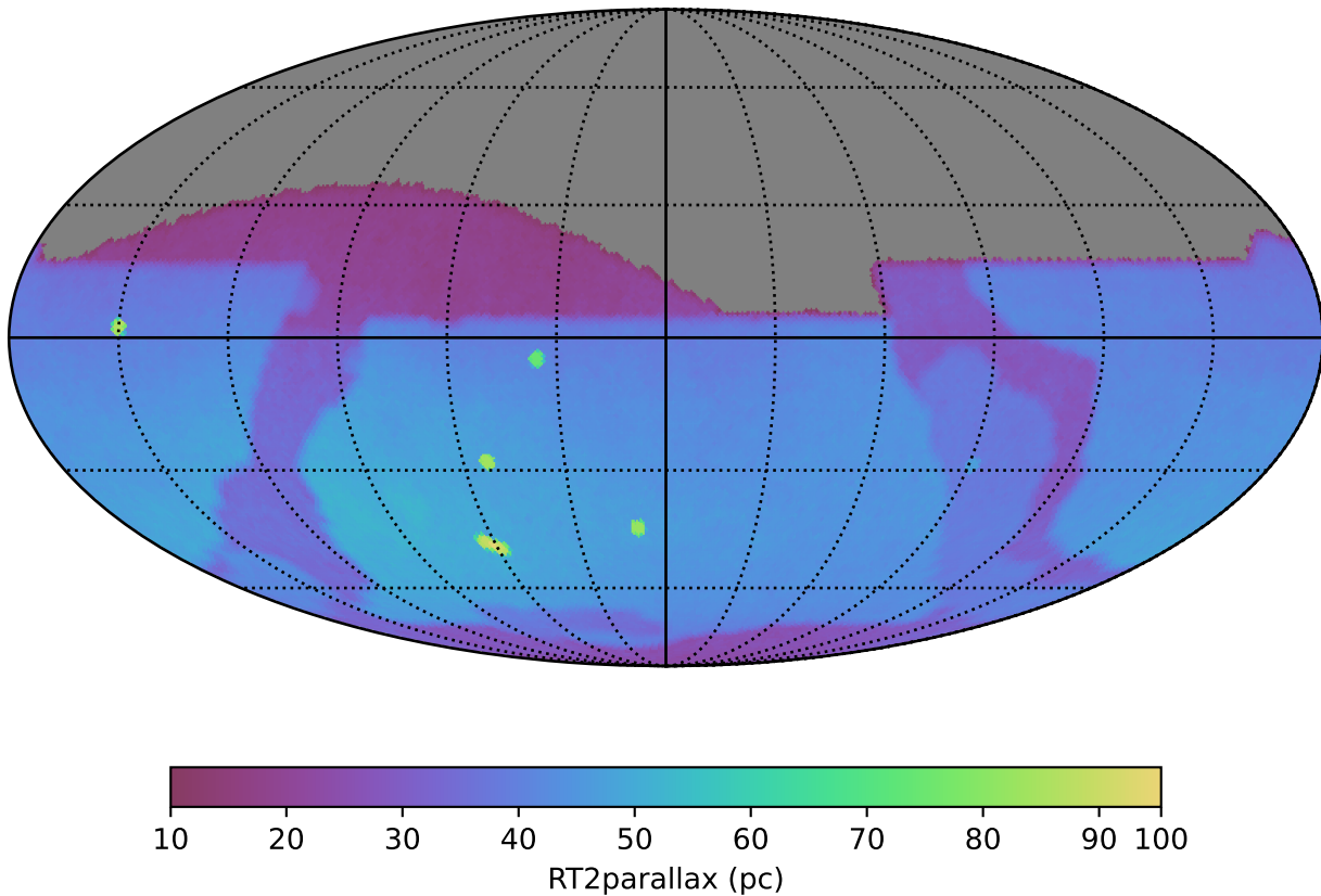
baseline_v5.3.0_10yrs : RT2parallax
