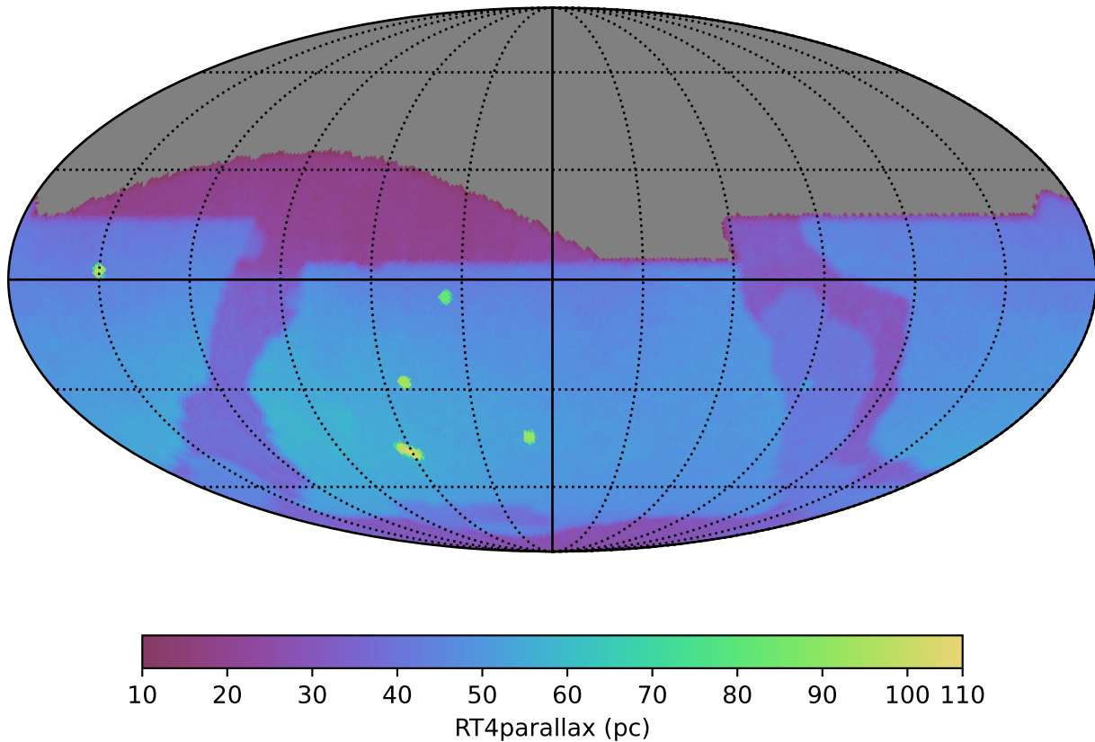
baseline_v5.3.0_10yrs : RT4parallax
