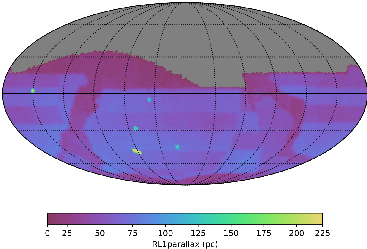
baseline_v5.0.0_10yrs night < 730: RL1parallax
