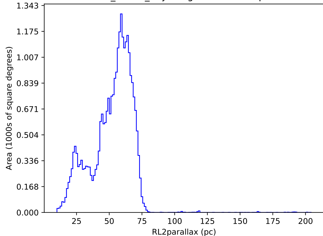
baseline_v5.0.0_10yrs night < 730: RL2parallax
