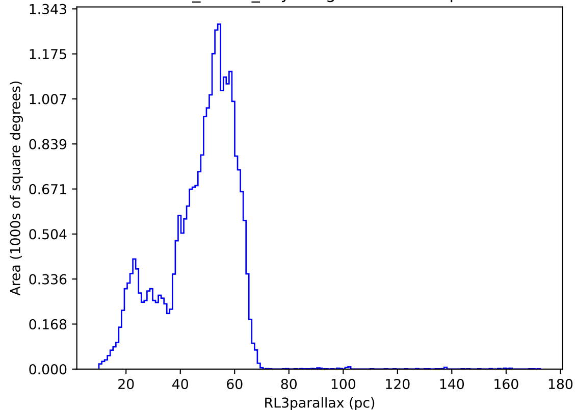
baseline_v5.0.0_10yrs night < 730: RL3parallax
