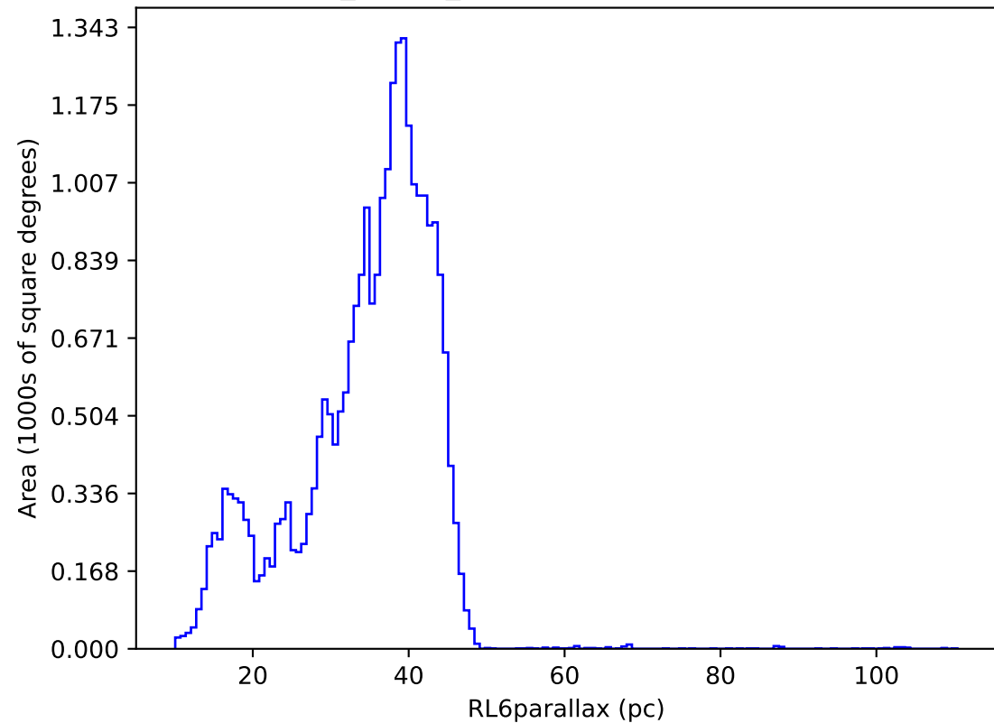
baseline_v5.0.0_10yrs night < 730: RL6parallax
