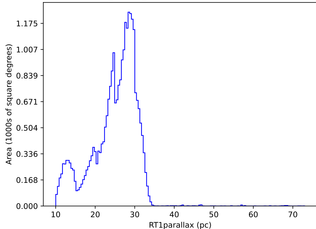
baseline_v5.0.0_10yrs night < 730: RT1parallax
