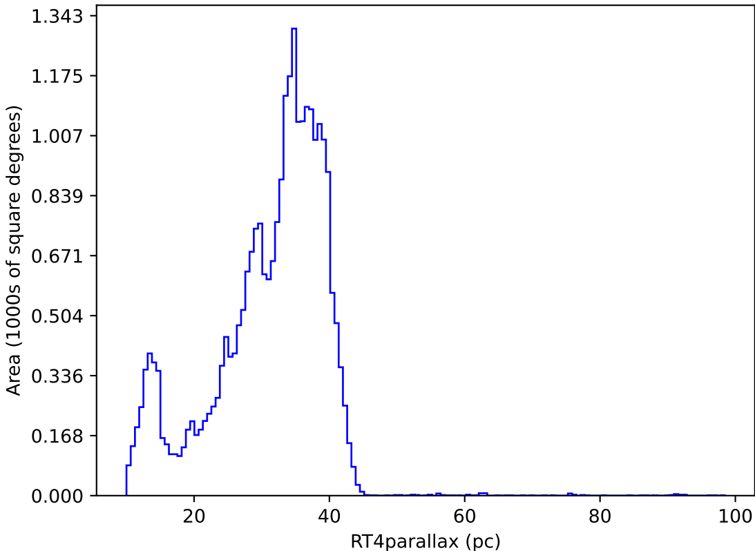
baseline_v5.0.0_10yrs night < 730: RT4parallax
