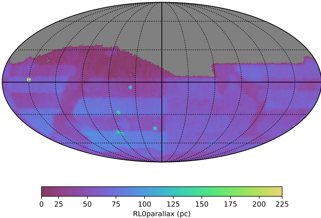
baseline_v5.3.0_10yrs night < 730: RL0parallax
