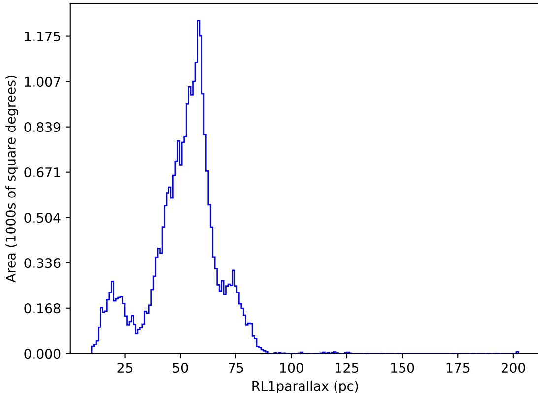
baseline_v5.3.0_10yrs night < 730: RL1parallax
