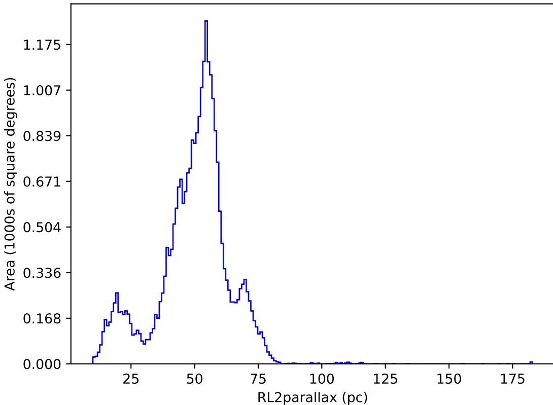
baseline_v5.3.0_10yrs night < 730: RL2parallax
