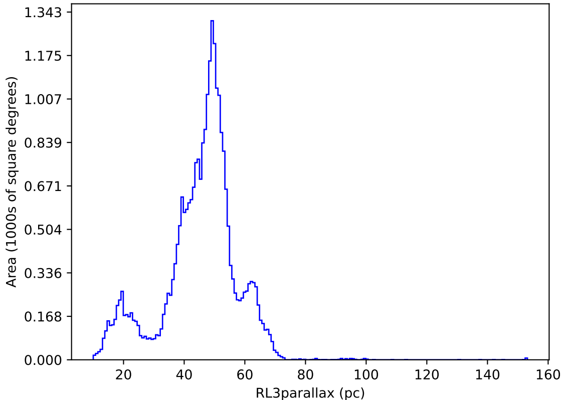
baseline_v5.3.0_10yrs night < 730: RL3parallax
