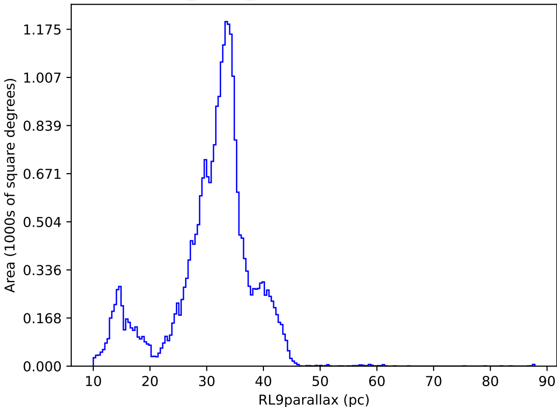
baseline_v5.3.0_10yrs night < 730: RL9parallax
